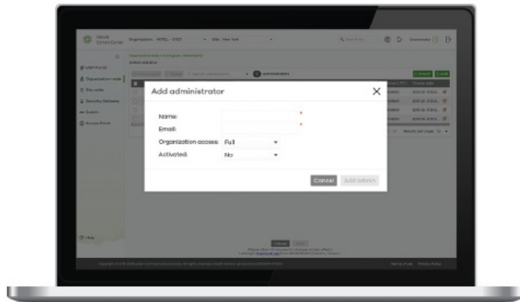
Role-based Administration
