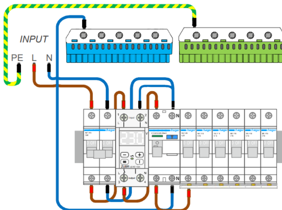
Scheme 3. Option of wiring diagram without a neutral bypass through D2
