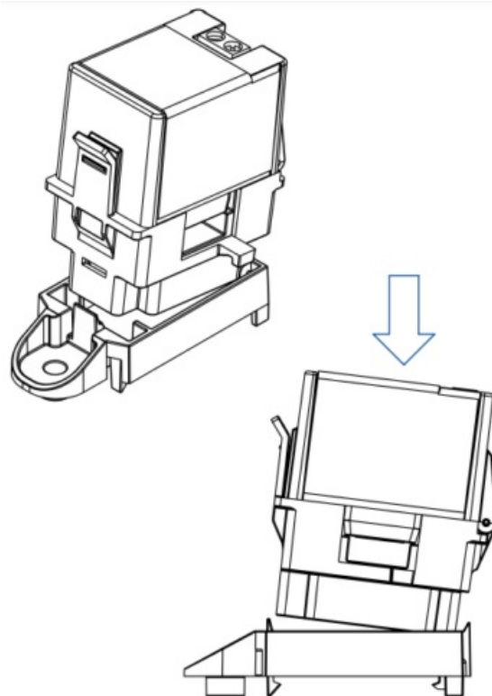
Figure 3: Mounting Foot Attachment
