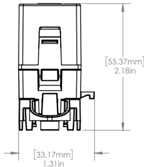
Figure 1: Enclosure Dimensions
