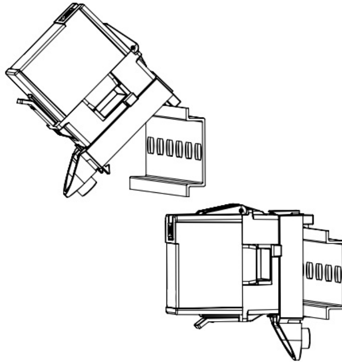
Figure 2: DIN Rail Installation
