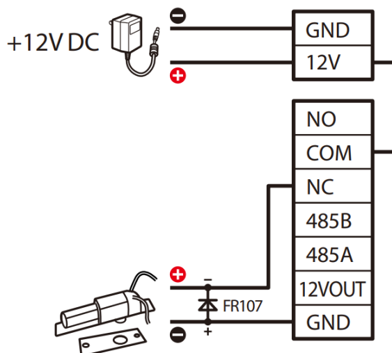
Normally Closed Lock
