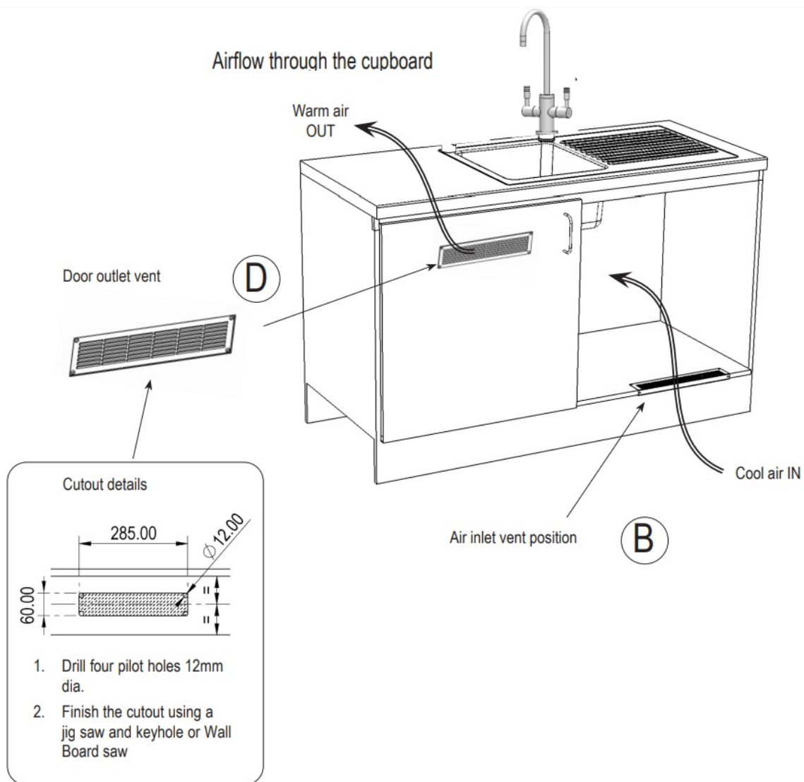
Typical Cut out procedure for B D
