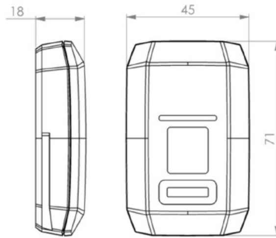
Figure 6 - Dimensions of the CorivaTag Plus
