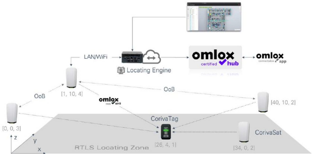
Figure 2 - Coriva RTLS Overview
