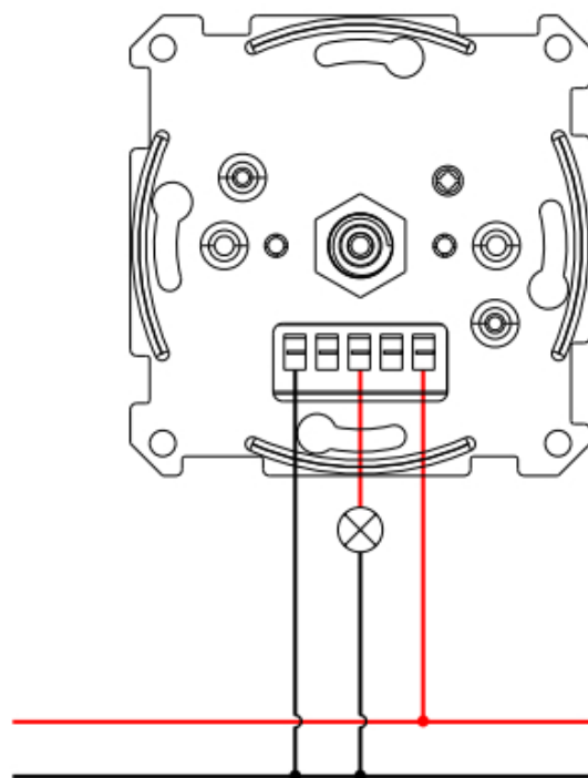
(2) 3-Wire Connection With Neutral Lead
