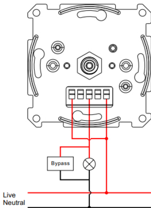
(1) 2-Wire Connection With No Neutral Lead
