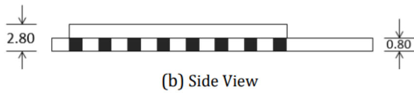
Fig.3.2 Size for XT-ZB6
