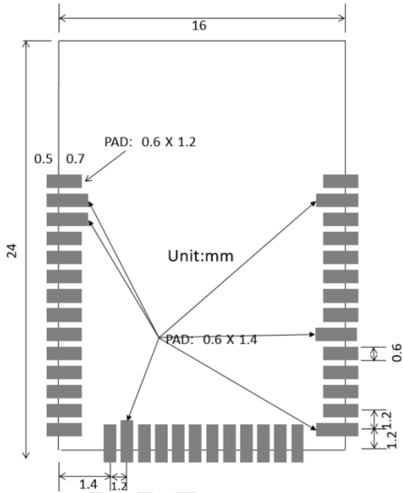
Fig.3.3 PCB Layout for XT-ZB6
