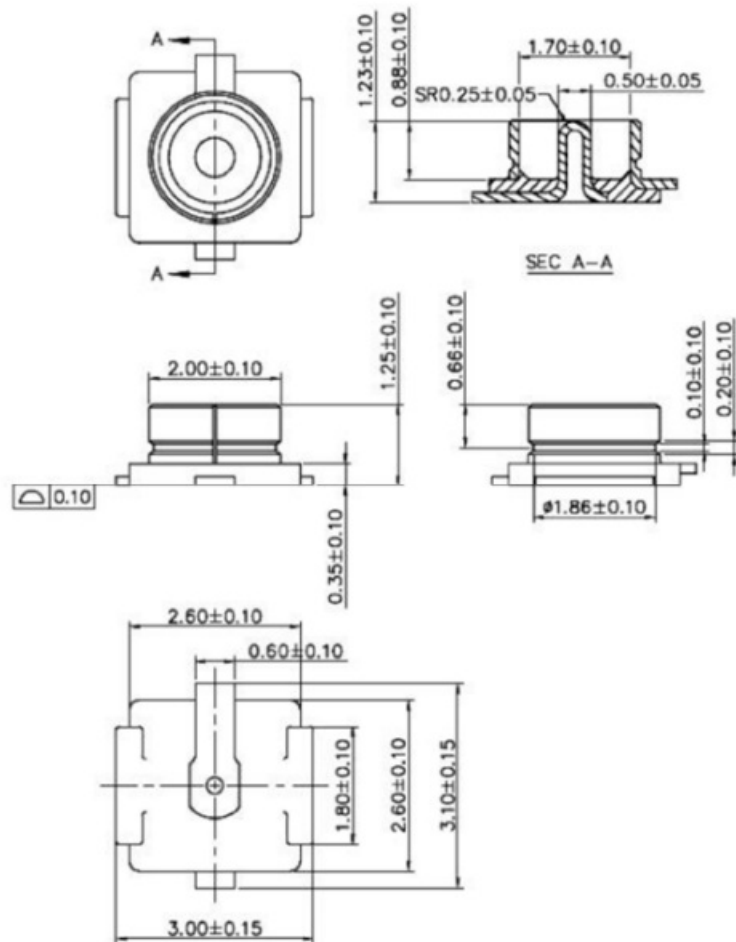
Fig.12.1 U.F.L RF Connector
