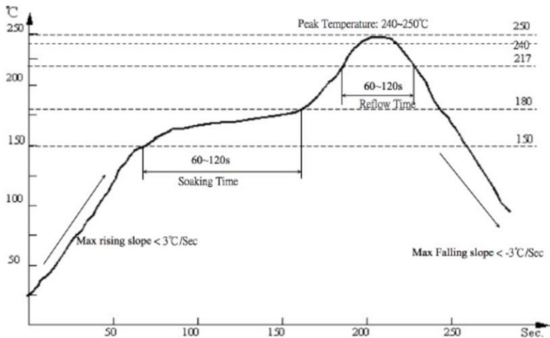
Fig.7.1 Recommended Reflow Profile
