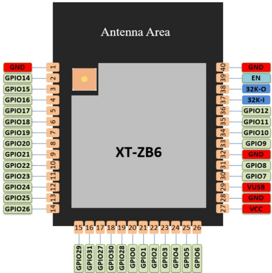
Fig.2.1 XT-ZB6 Pin Definition
