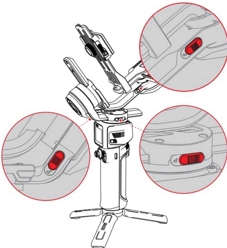
Locked state for installation
