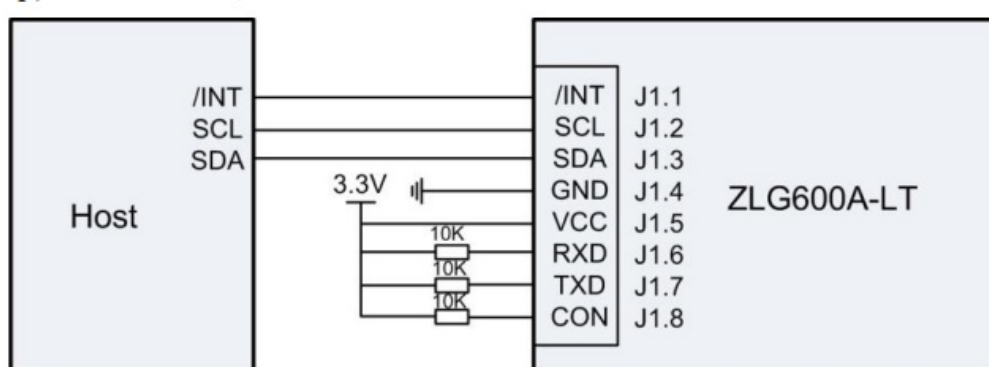
Figure 4 Typical application of automatic detection of I2C
