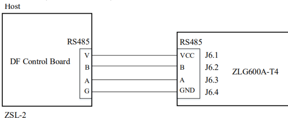
Figure 6 ZSL-2 host RS485 interface typical application
