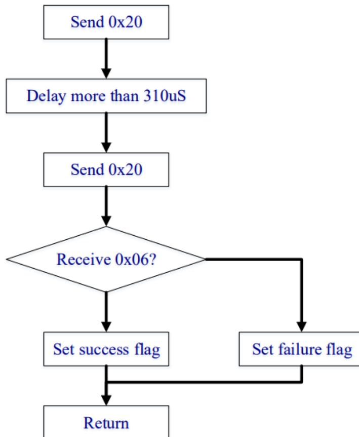
Figure 3 Determine the communication baud rate
