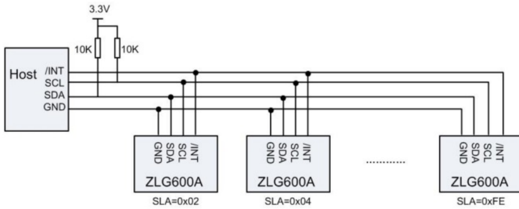
Figure 5 I2C multi-slave connection diagram
