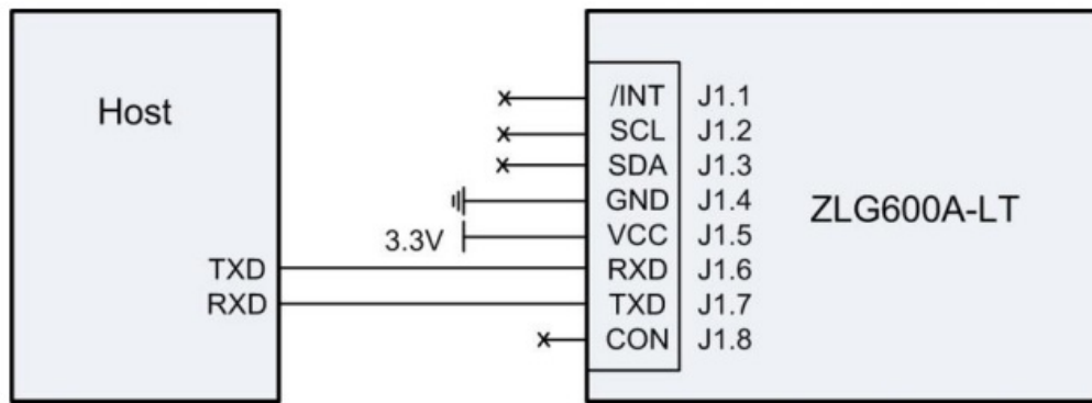
Figure 2 Automatic detection mode Typical application of UART
