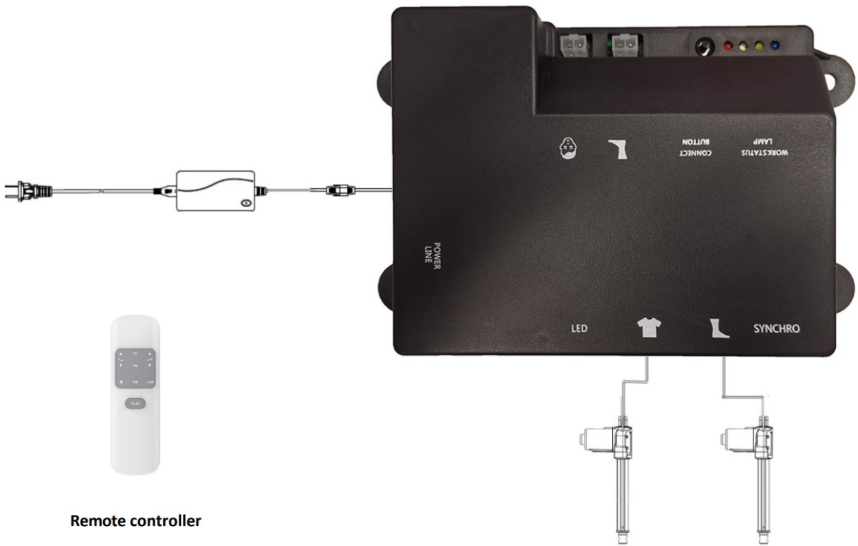
Control box
