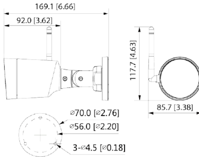
Figure 4-2 Dimensions (mm [inch])
