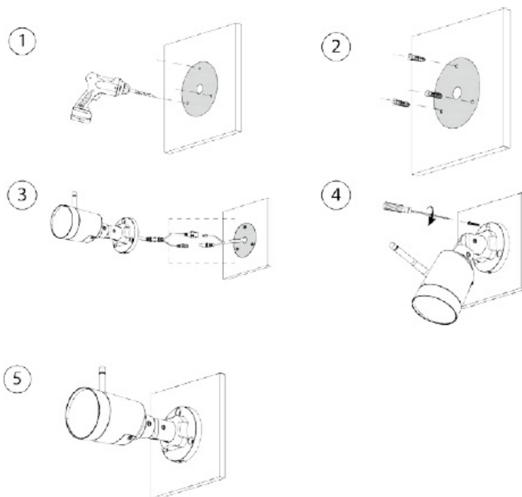
Figure 4-6 Cable going through the mounting surface
