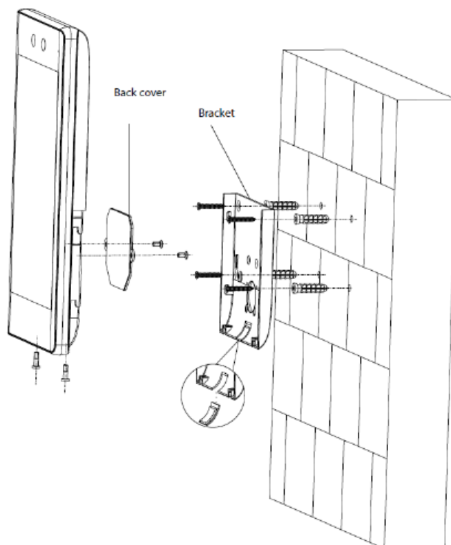
Figure 2-6 Wall mount
