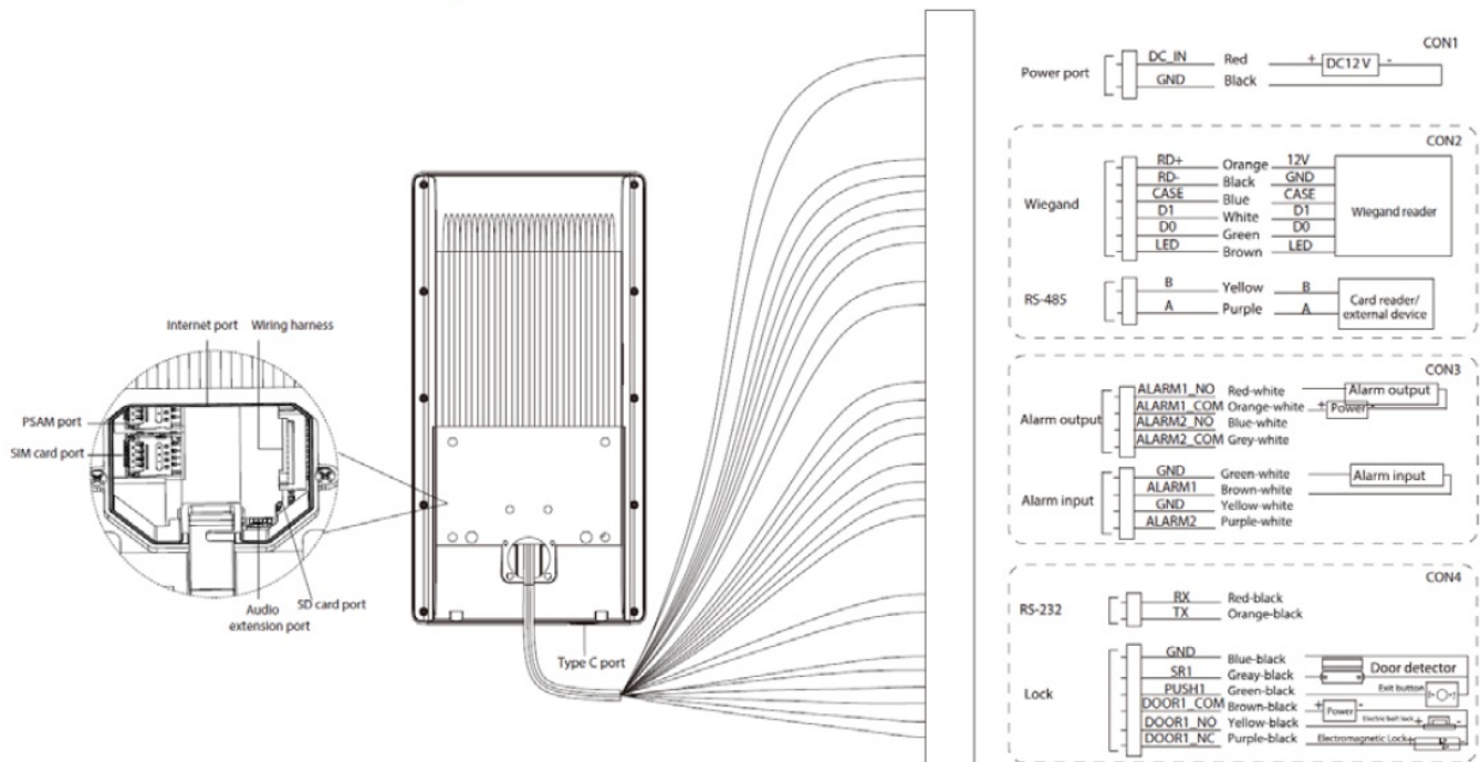
Figure 2-1 Cable connections
