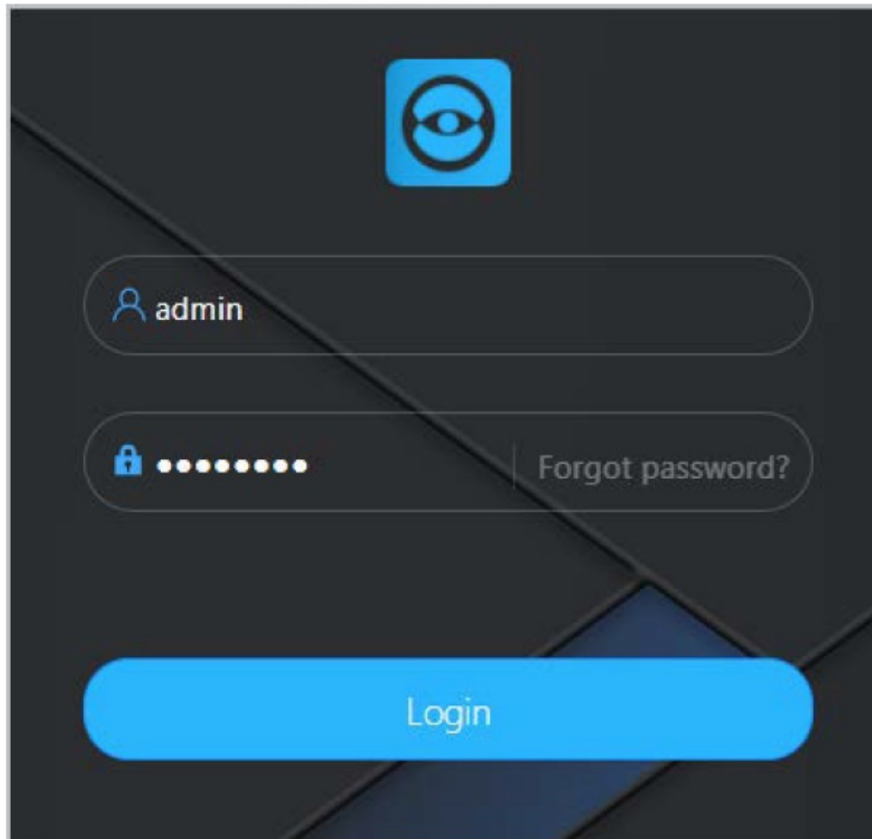
Figure 4-2 Login
