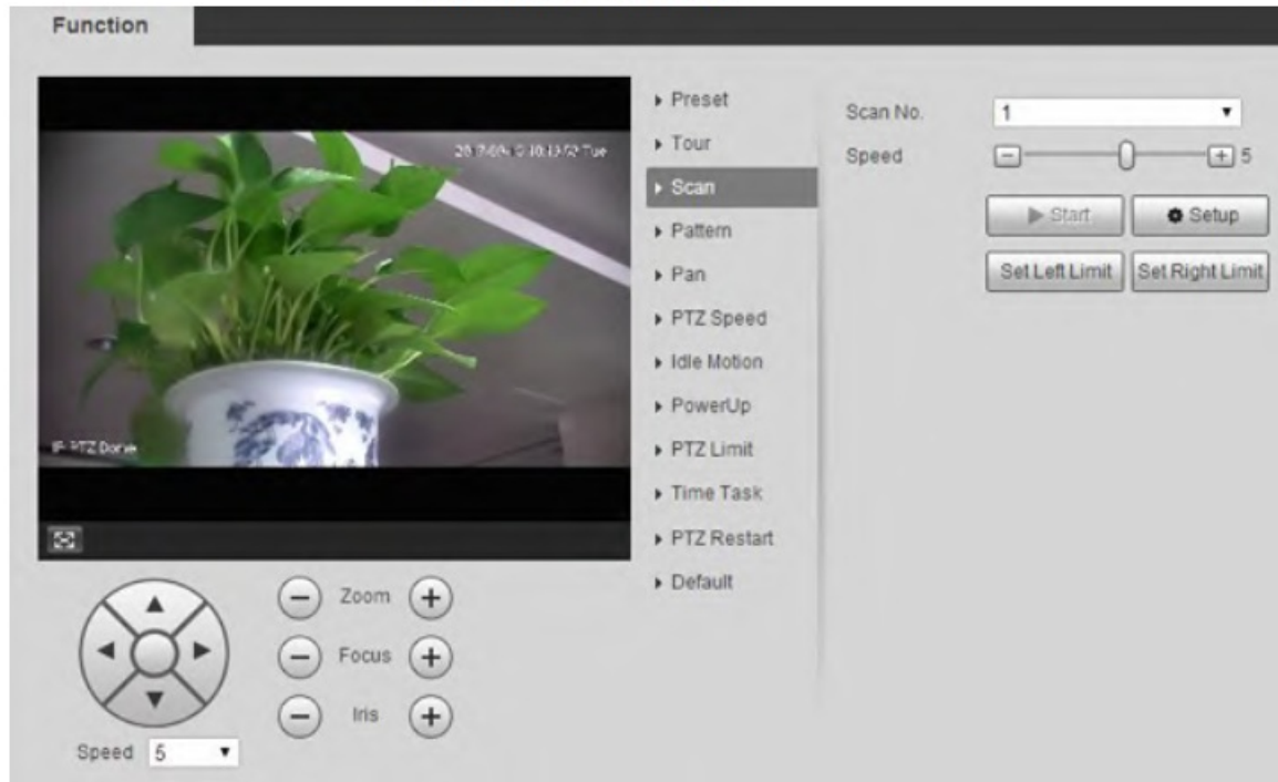
Figure 5-71 Scan settings
