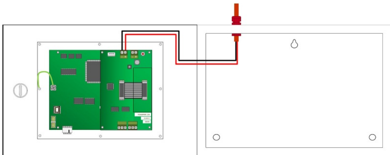
Figure 3: 28V DC wiring
