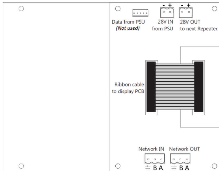
Figure 2: Termination PCB Layout
