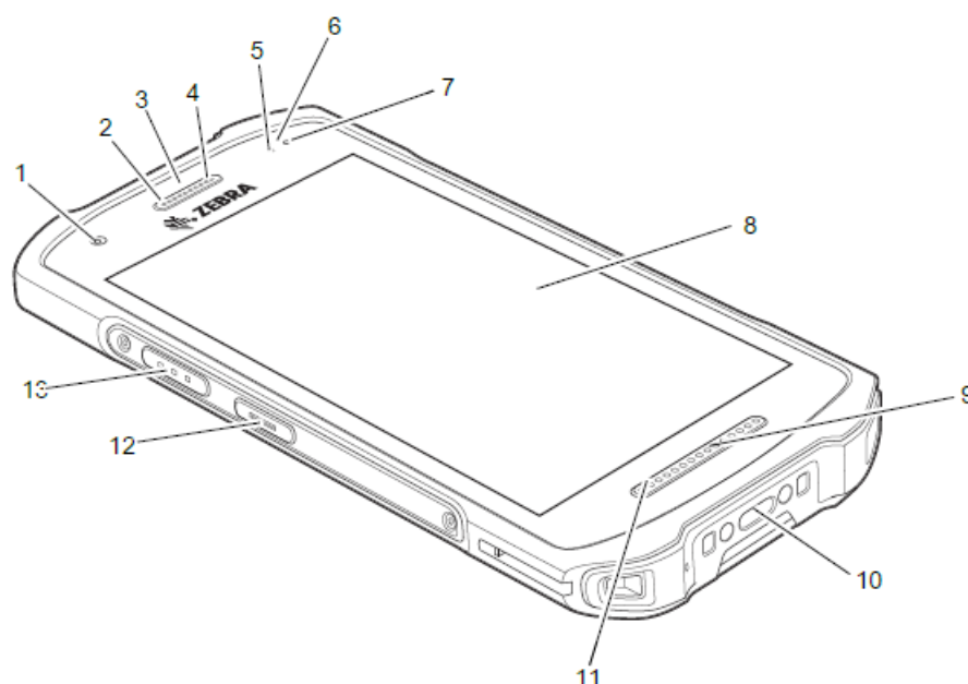
Figure 1 Front View
