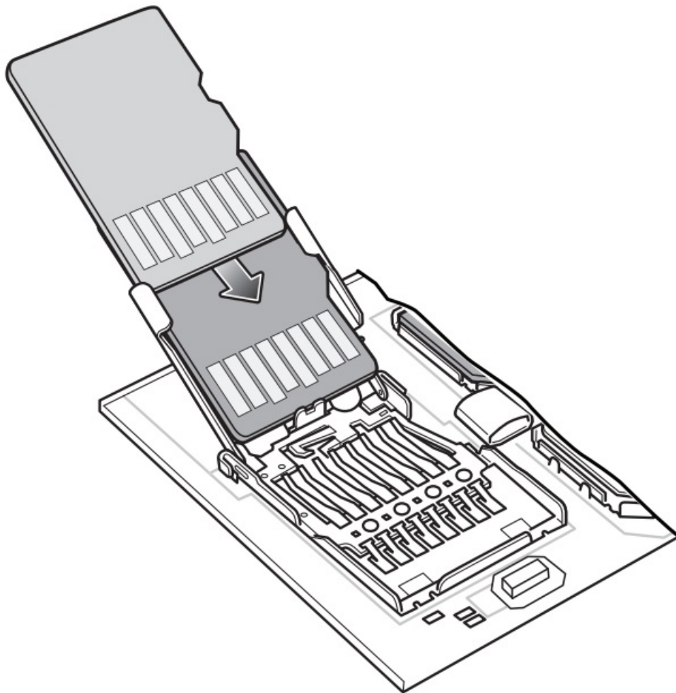
Figure 15 Insert microSD Card into Holder
