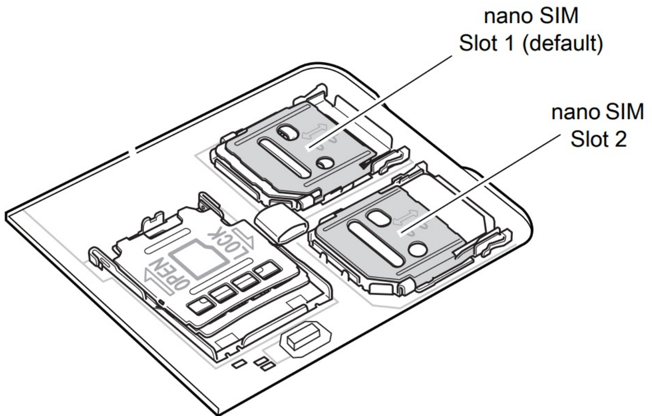
Figure 3 TC77 SIM Slot Locations
