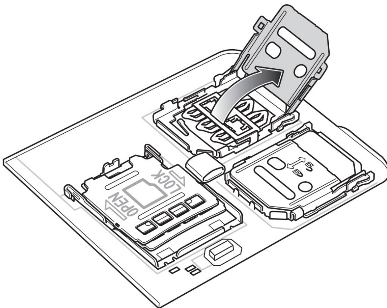
Figure 5 Lift the SIM Card Holder
