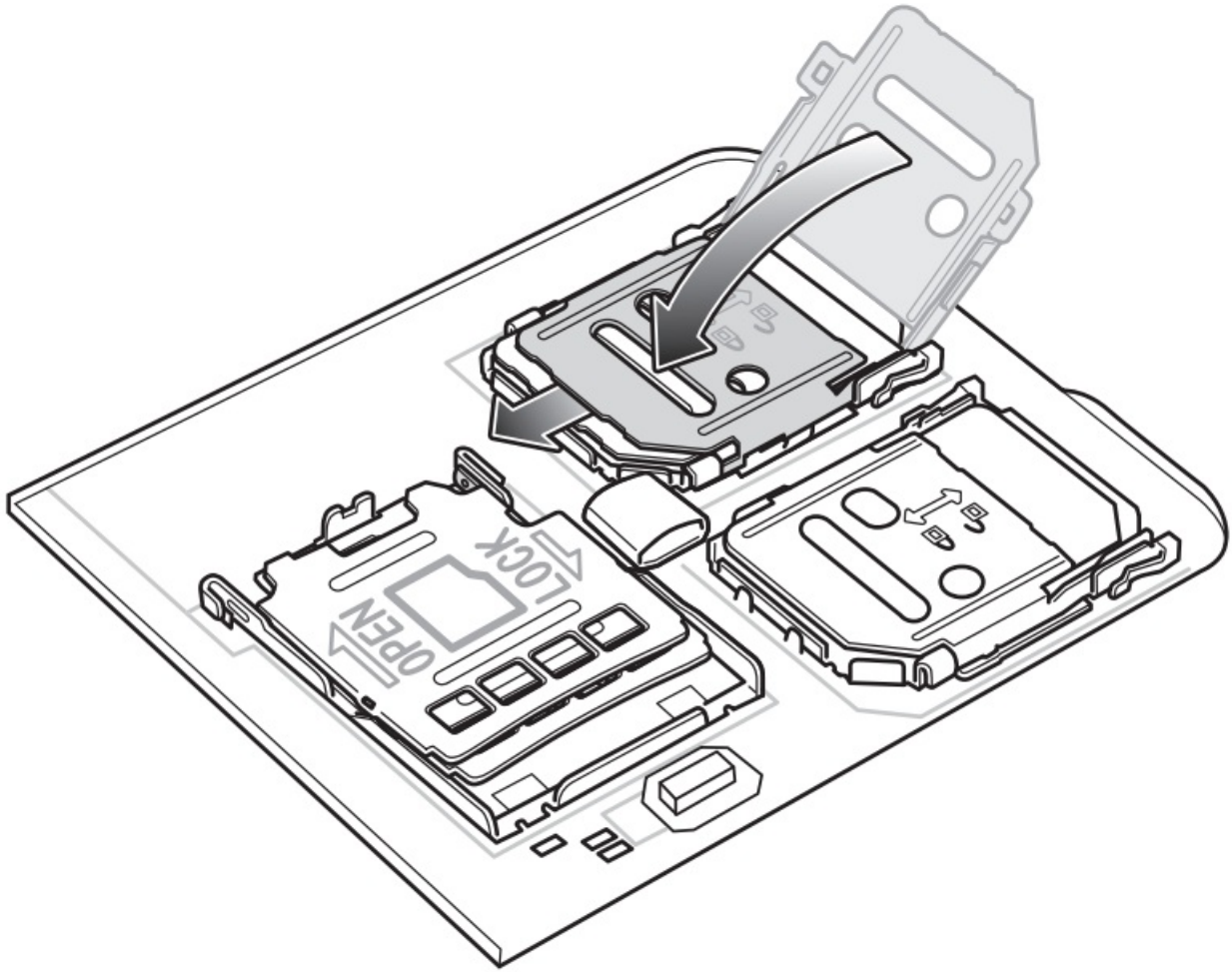
Figure 8 Replace Access Door
