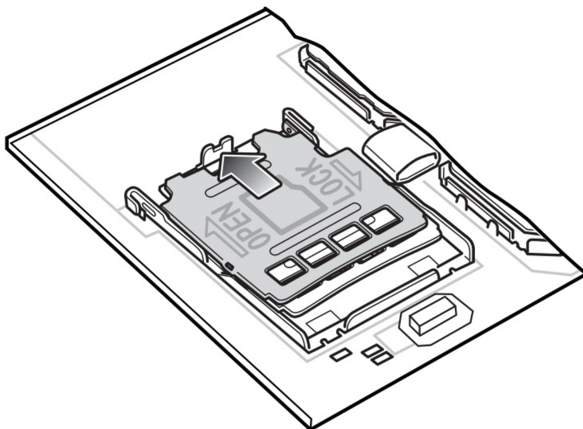
Figure 13 Open microSD Card Holder
