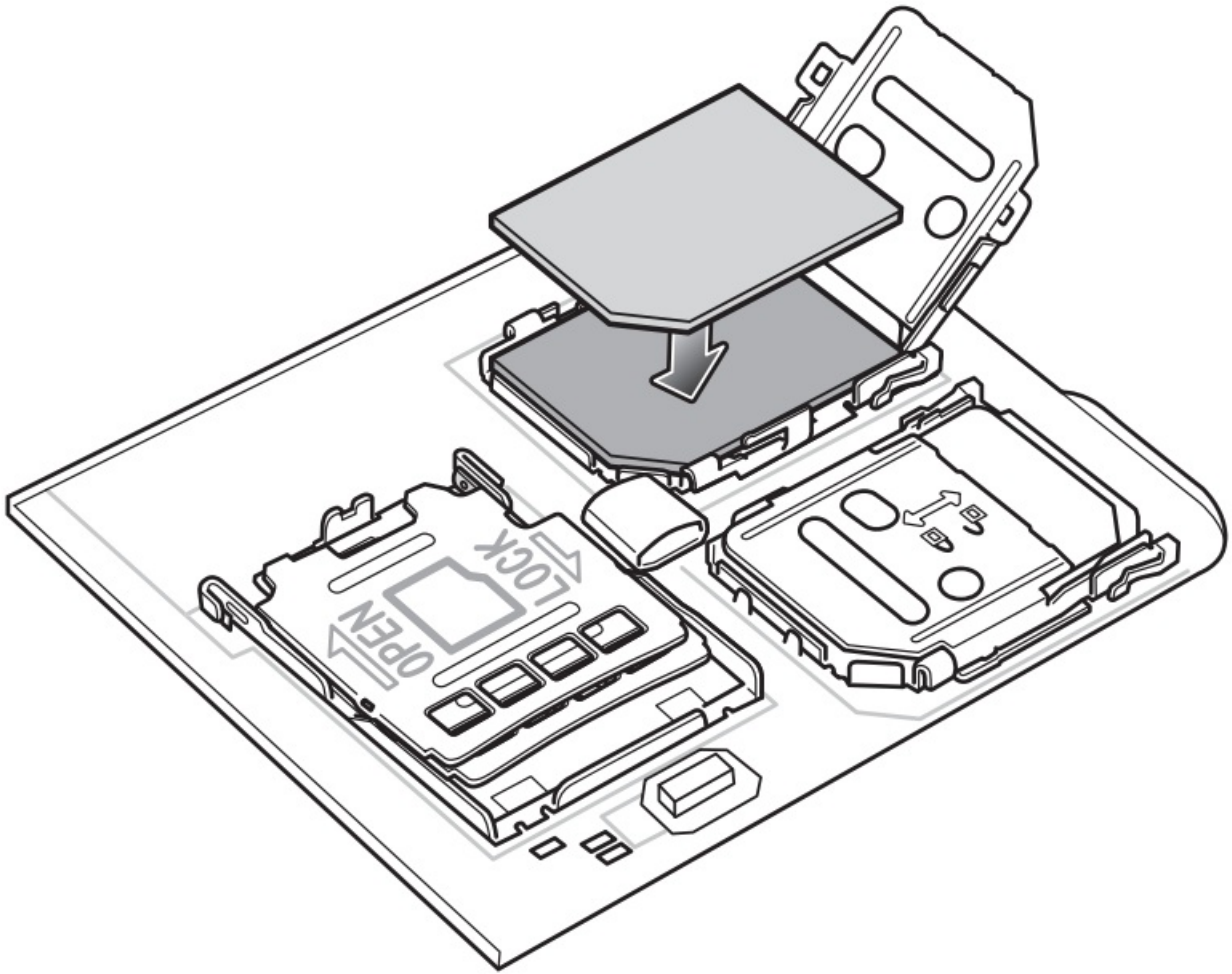
Figure 6 Place SIM Card in Holder
