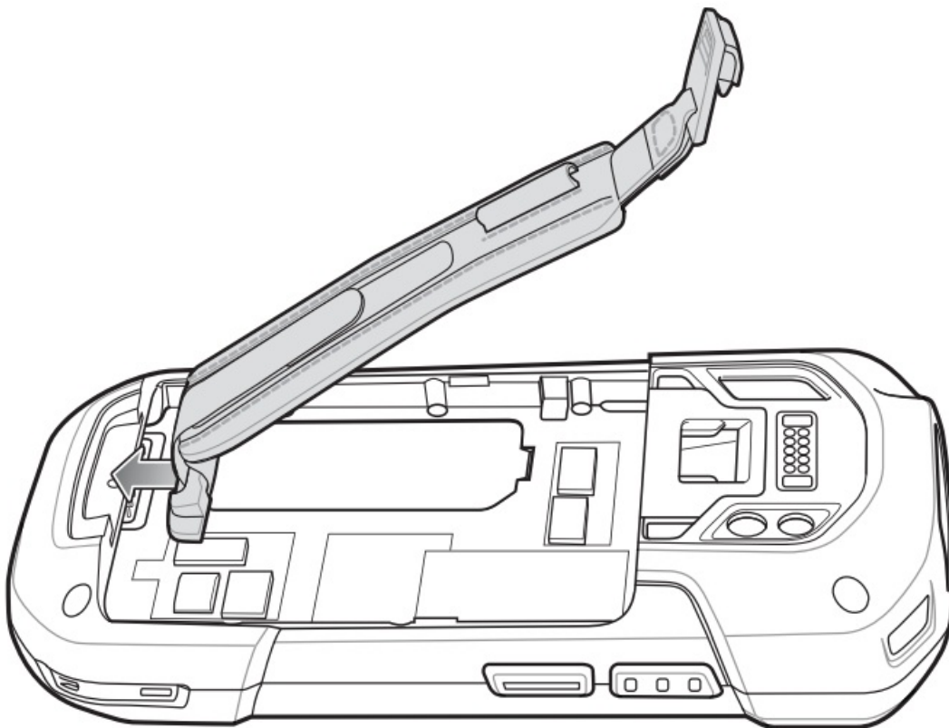
Figure 19 Insert Hand Strap
