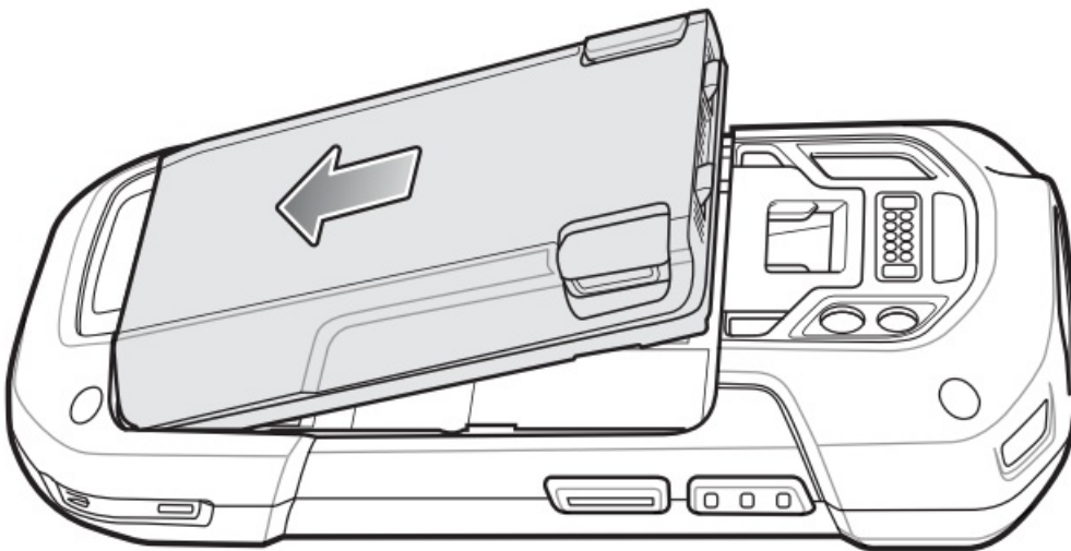
Figure 23 Insert Bottom of Battery into Battery Compartment
