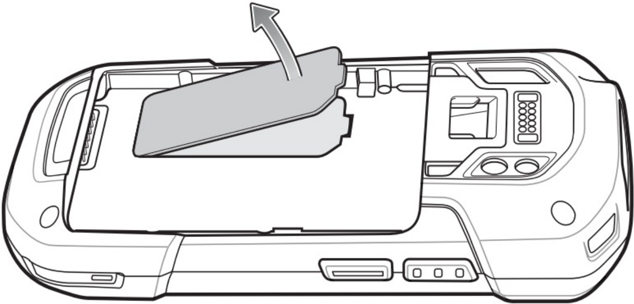
Figure 9 Remove Access Door
