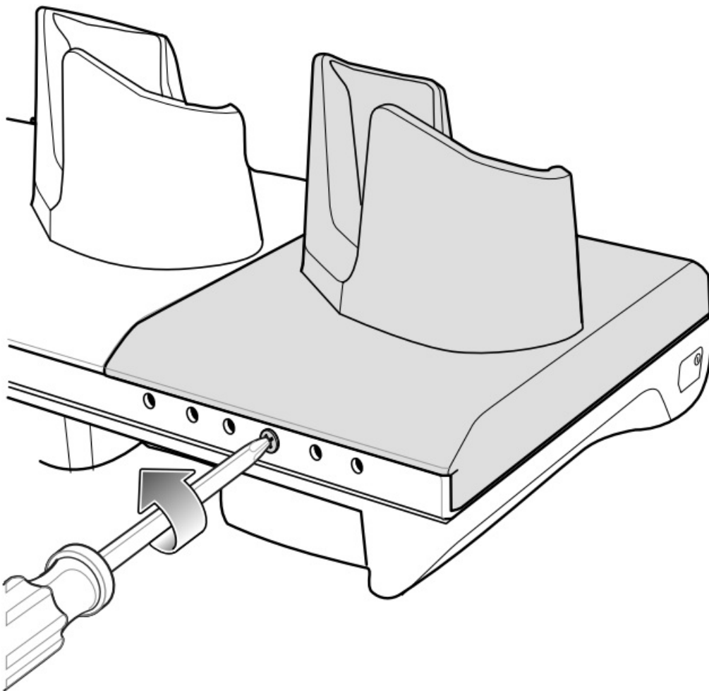
Figure 44 Remove Cup
