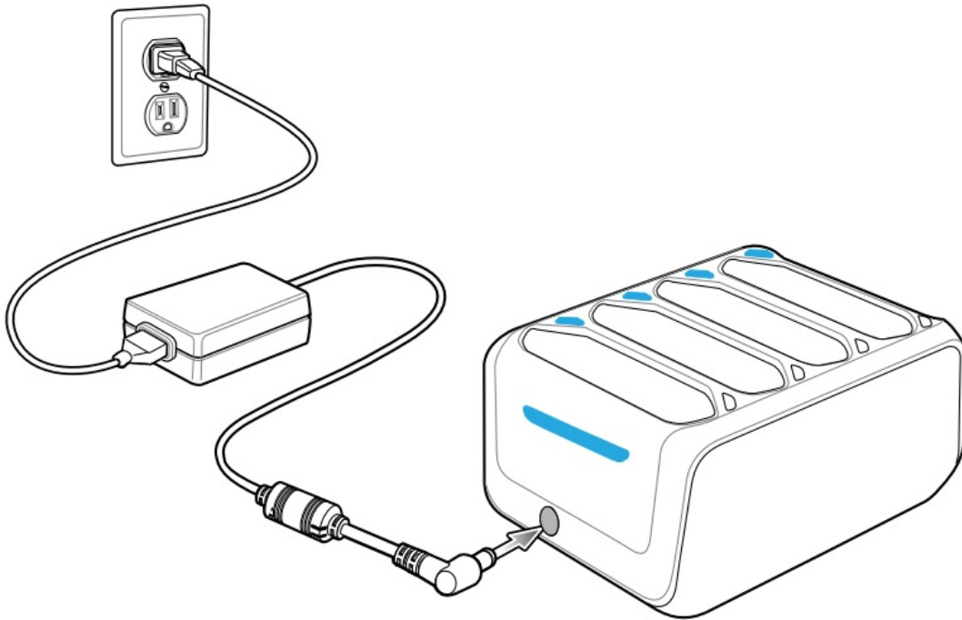
Figure 46 Four Slot Battery Charger Power Setup
