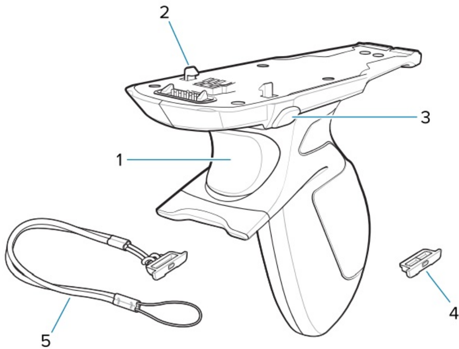
Figure 49 Trigger Handle
