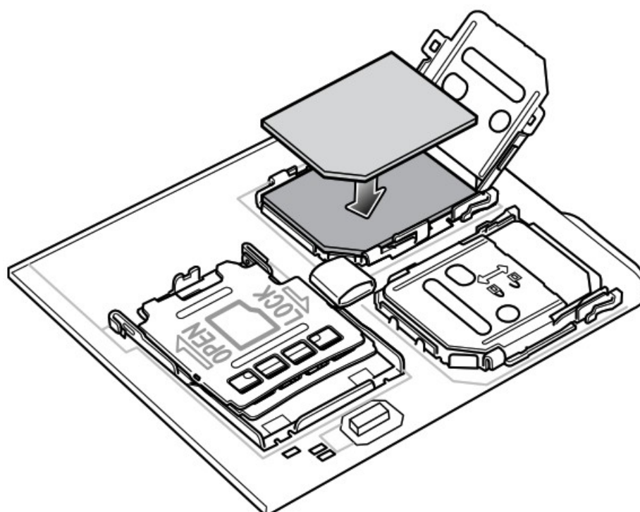
Figure 7 Insert Nano SIM Card
