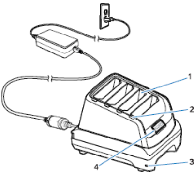
Figure 6 4-Slot Battery Charger
