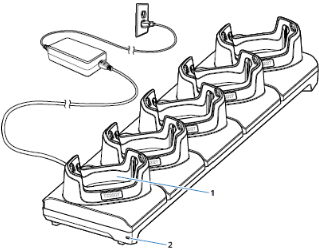
Figure 7 5-Slot Charge Only Cradle
