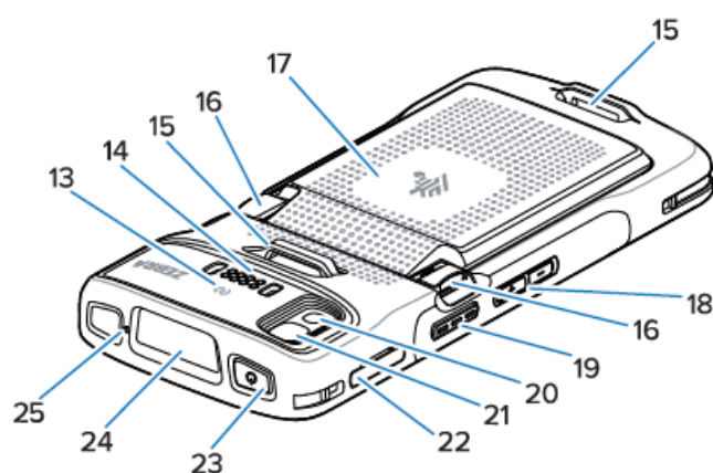
Figure 2 Rear View
