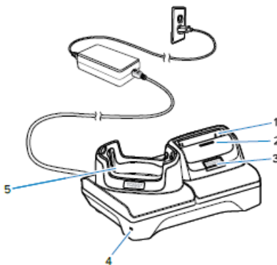
Figure 5 1-Slot Cradle with Spare Battery Slot
