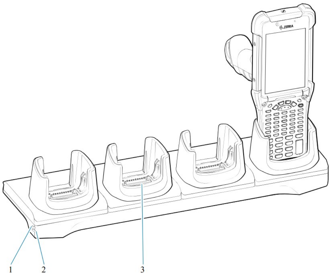
Figure 6 4-Slot Ethernet ShareCradle
