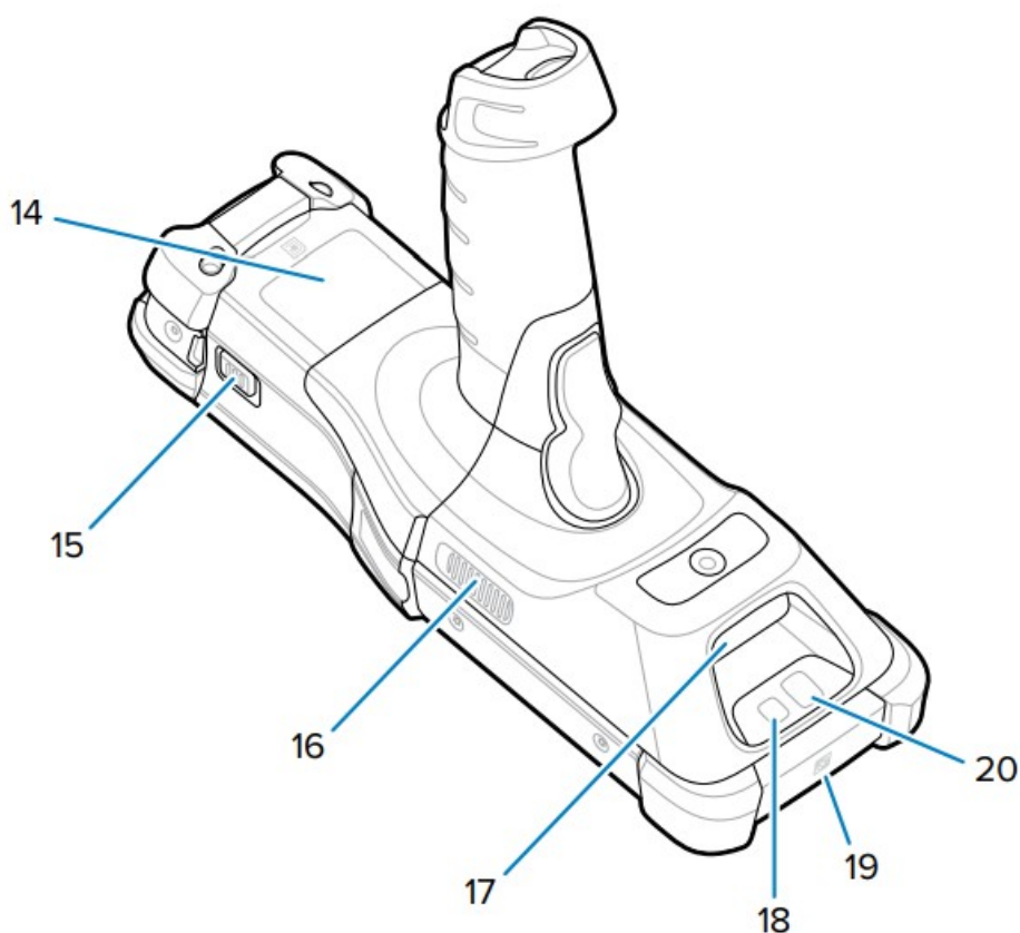
Figure 2 Bottom View
