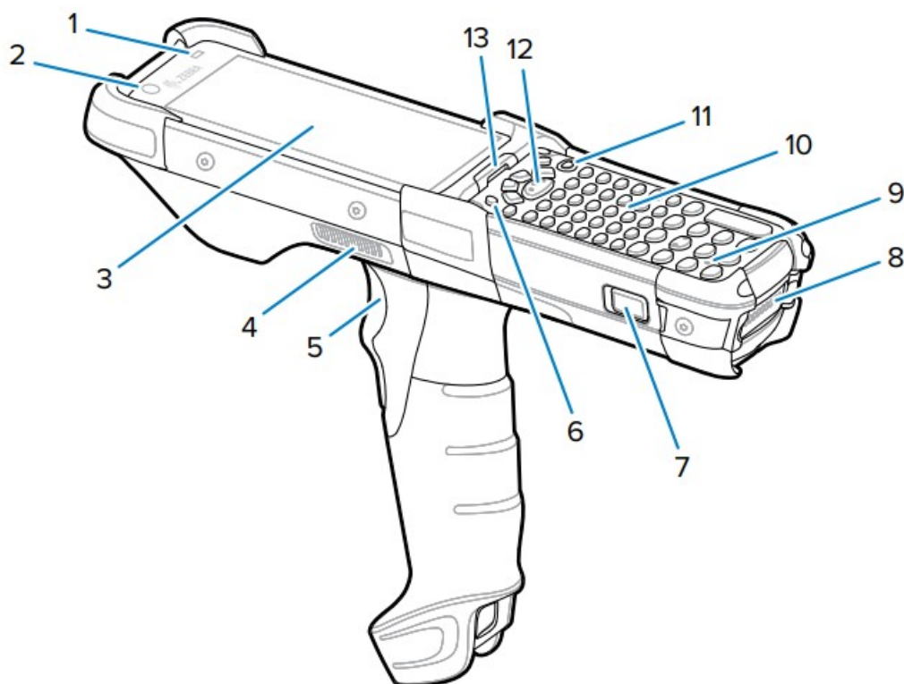
Figure 1 Top View
