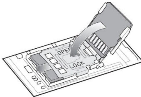
Figure 9 Close and Lock microSD Card in Holder
