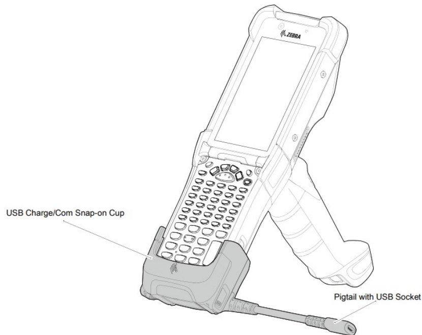
Figure 21 USB Charge/Com Snap-on Cup
