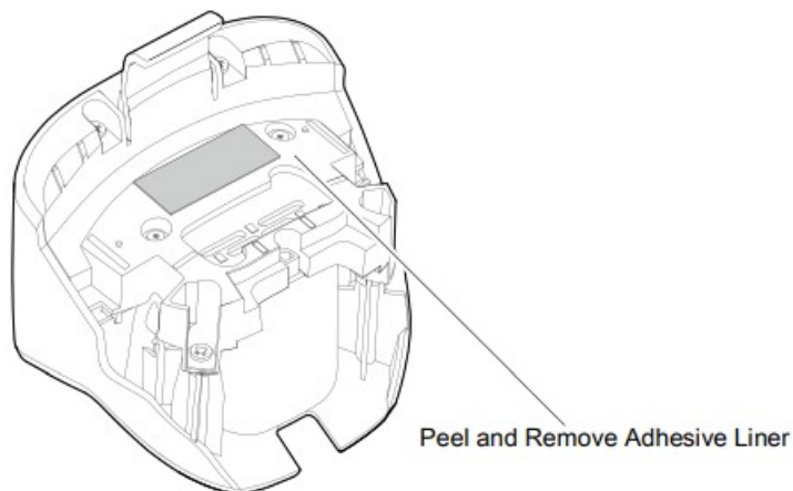
Figure 25 Peel and Remove Adhesive
