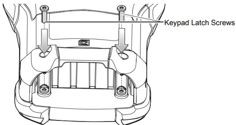
Figure 13 Replace Keypad Latch Screws
