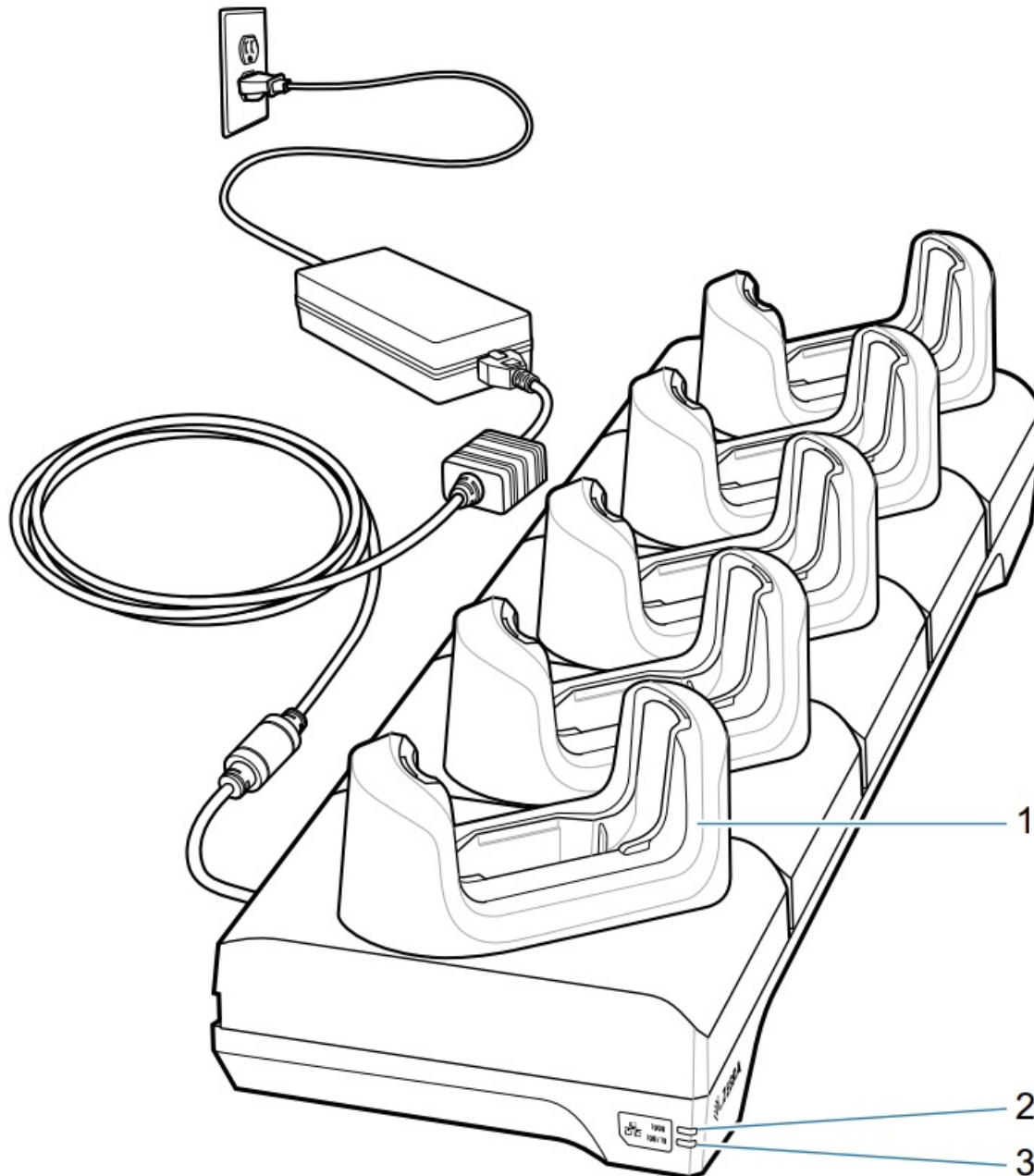
Figure 7 5-Slot Ethernet Cradle
