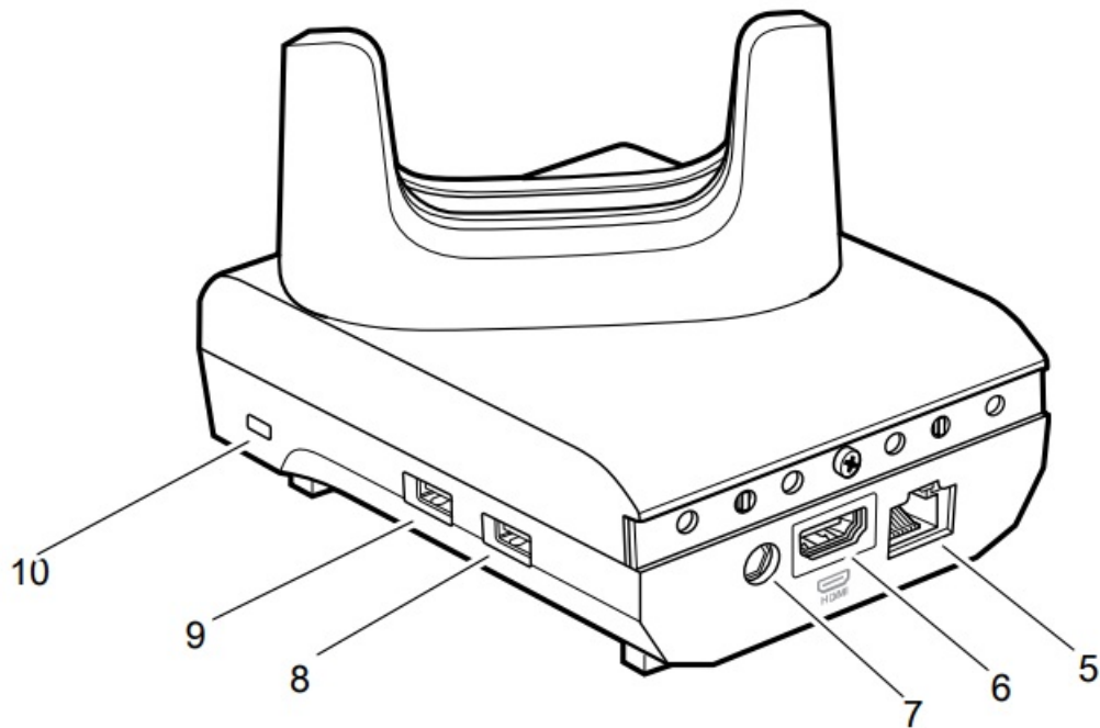
Figure 6 Rear Right View
