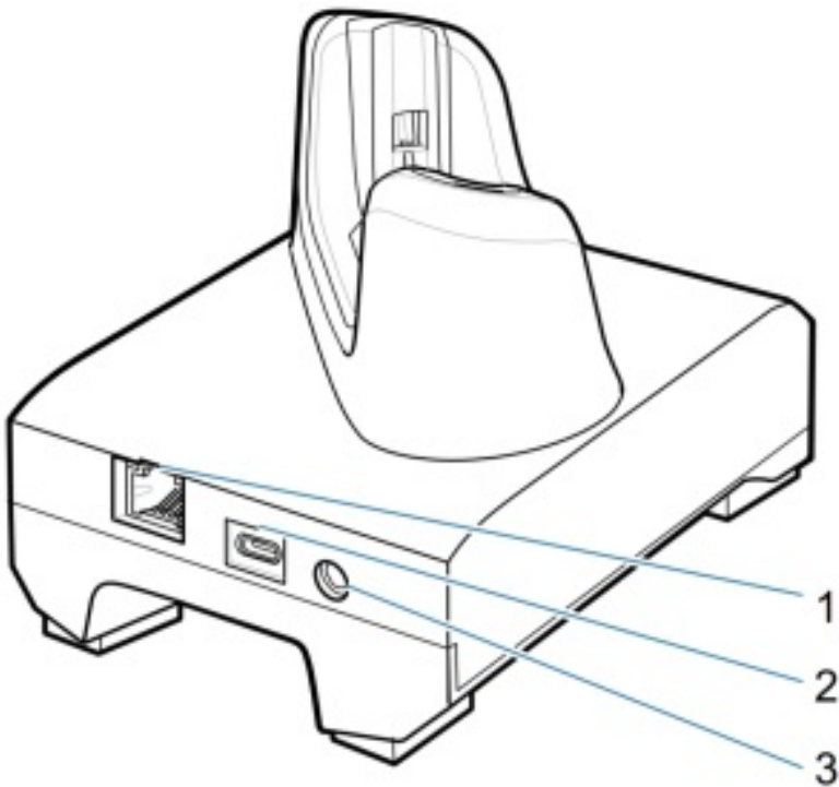
Figure 4 Back View
