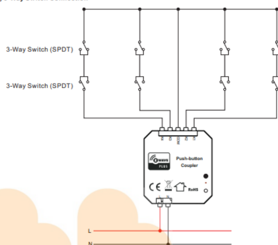
(3) 3-Way Switch Connection
