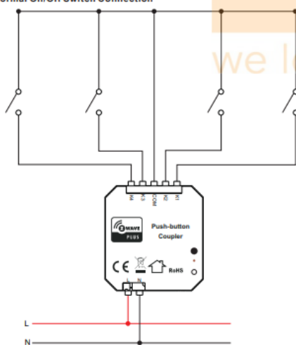
(2) Normal On/Off Switch Connection
