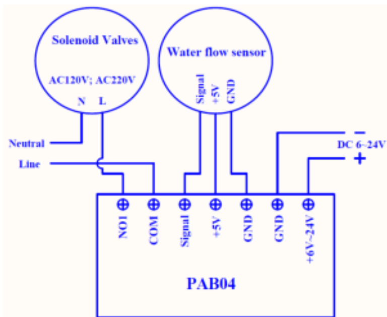
Fig 2. PAB04 Assembling & Wiring
