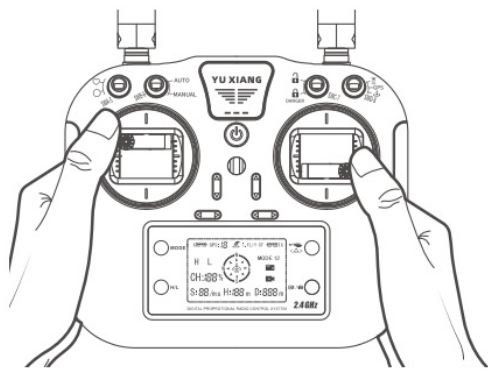
MODE2 (American-hand gyroscope calibration)
