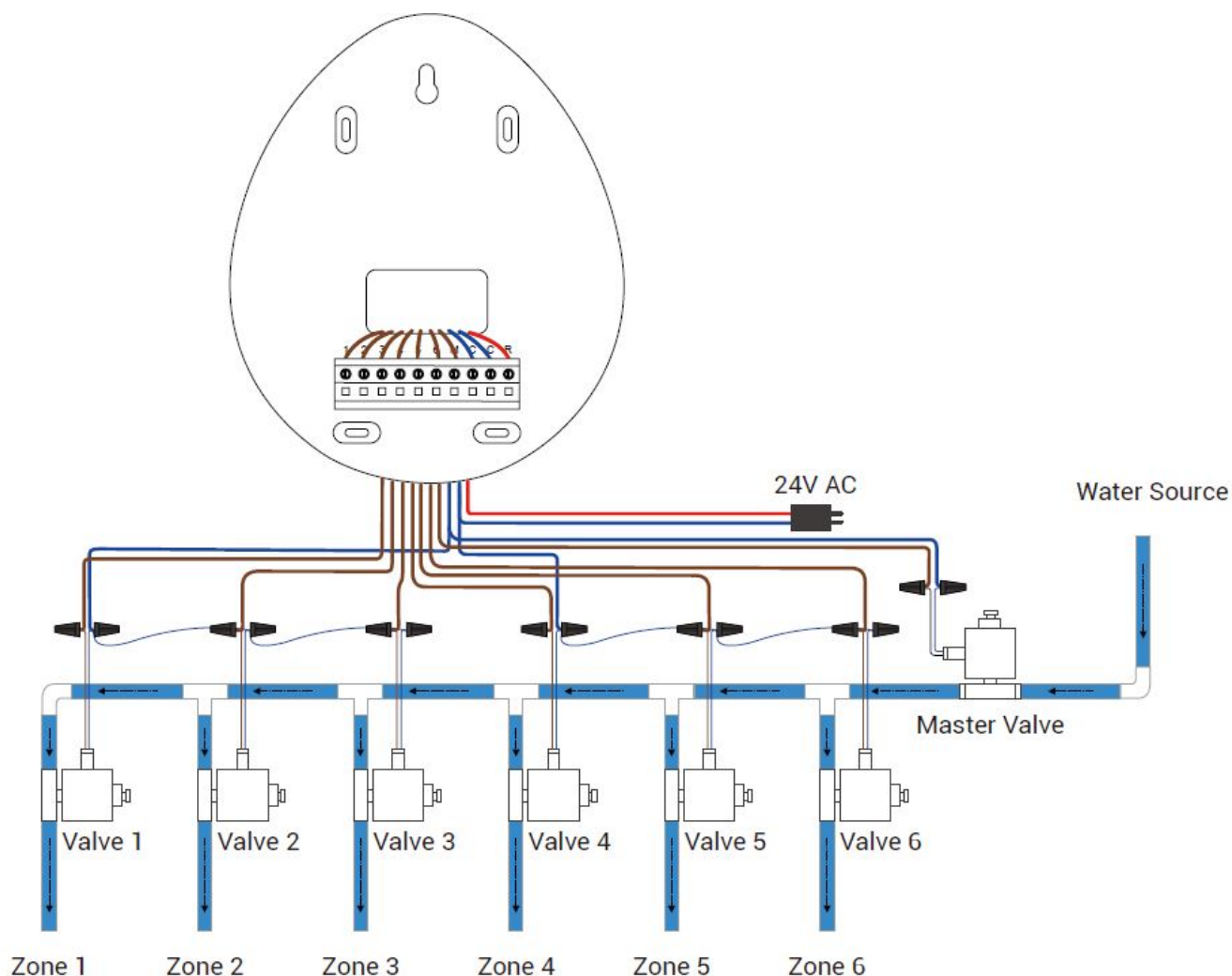
Wiring Diagram
