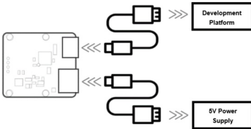
FIG 3 YDLIDAR GS5 AUXILIARY POWER SUPPLY
