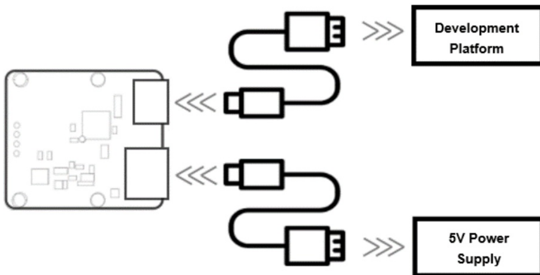
FIG 3 YDLIDAR GS2 AUXILIARY POWER SUPPLY
