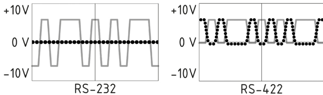
Figure 2. (a) RS-232 and (b) RS-422
