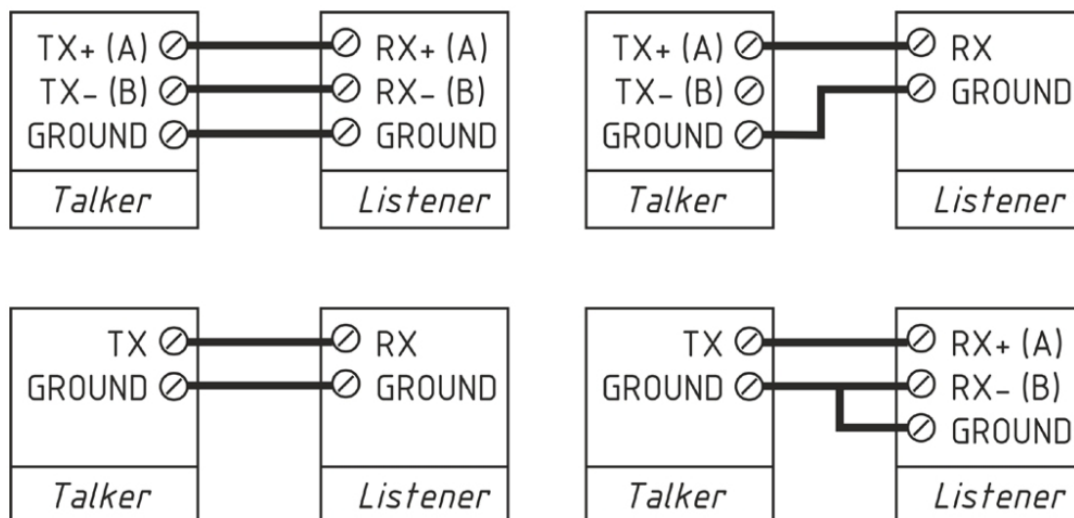
Figure 3. Connection of NMEA 0183 devices
