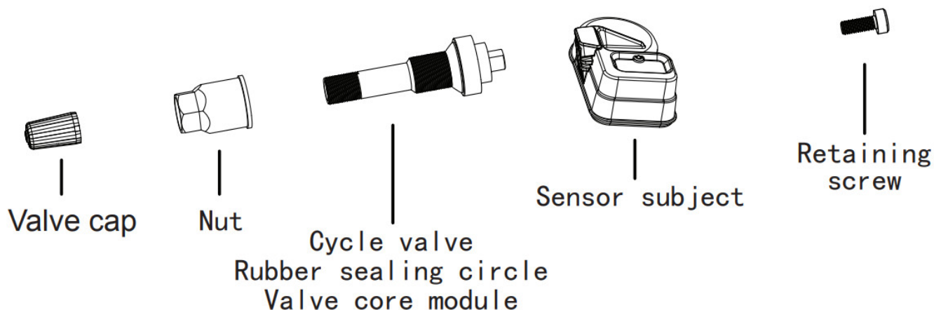
TS100 tire pressure sensor technical parameters
