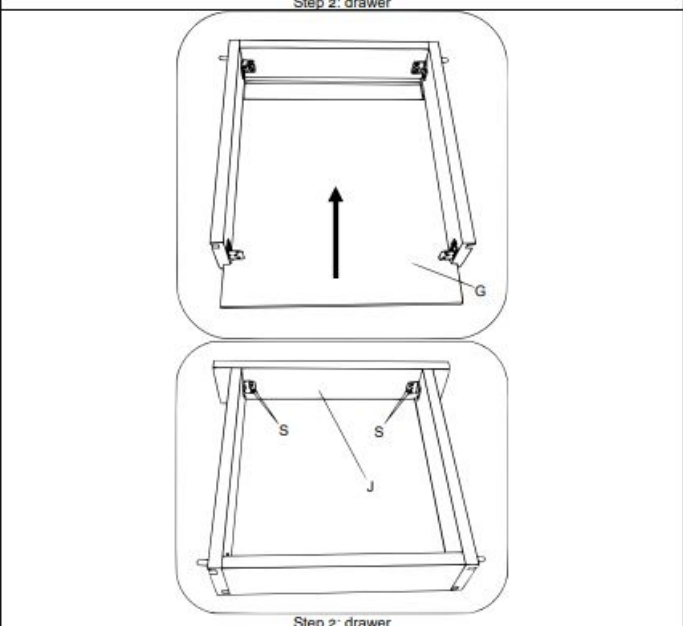
Step 2: drawer
