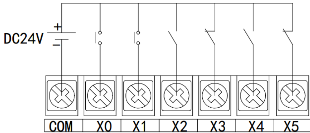
Switch button wiring
