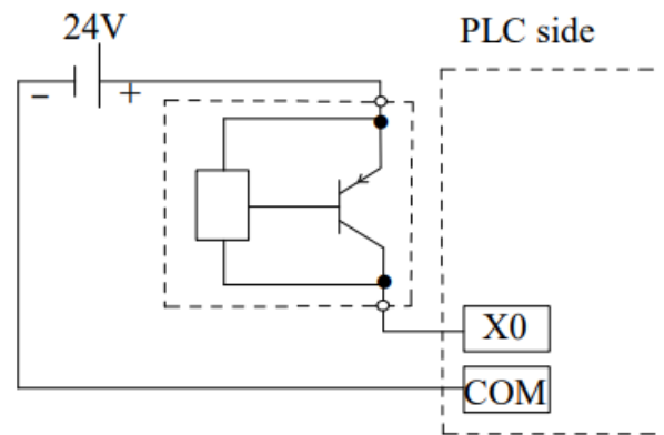
2-wire (PNP) proximity switch wiring
