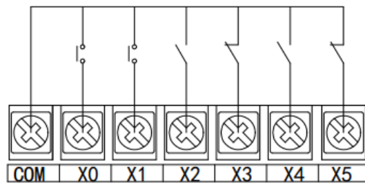
Switch button wiring
