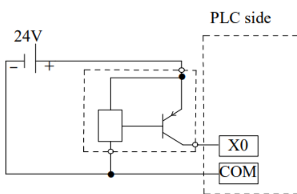
3-wire (PNP) proximity switch wiring
