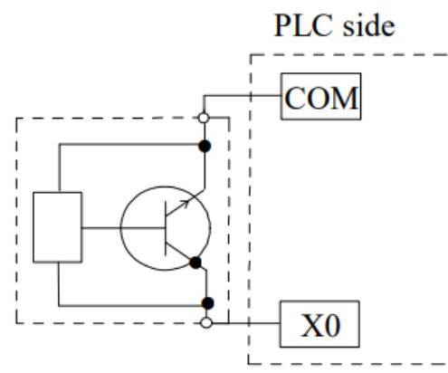
2-wire (NPN) proximity switch wiring
