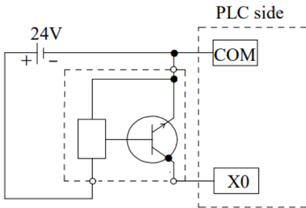
3-wire (NPN) proximity switch wiring
