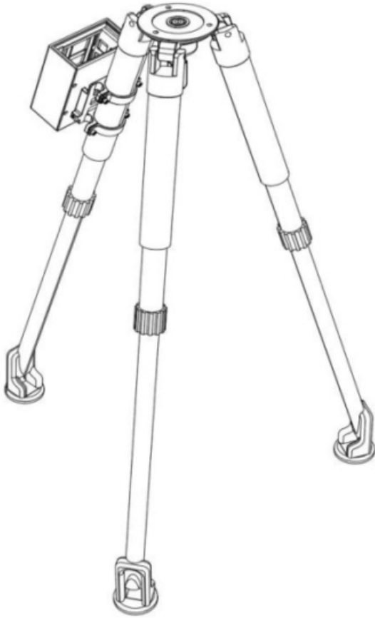
Figure 2-7 HD TLS360 system carbon fiber tripod
