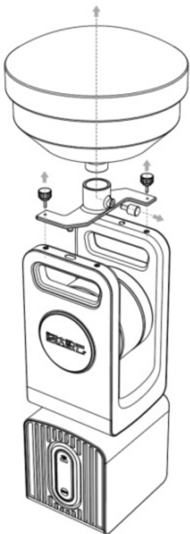
Figure 3-2.6 Disassembly diagram of HD TLS360 system RTK
