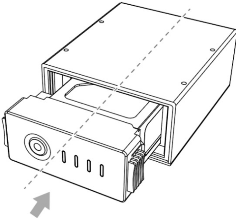
Figure 3-2.1 Battery Installation
