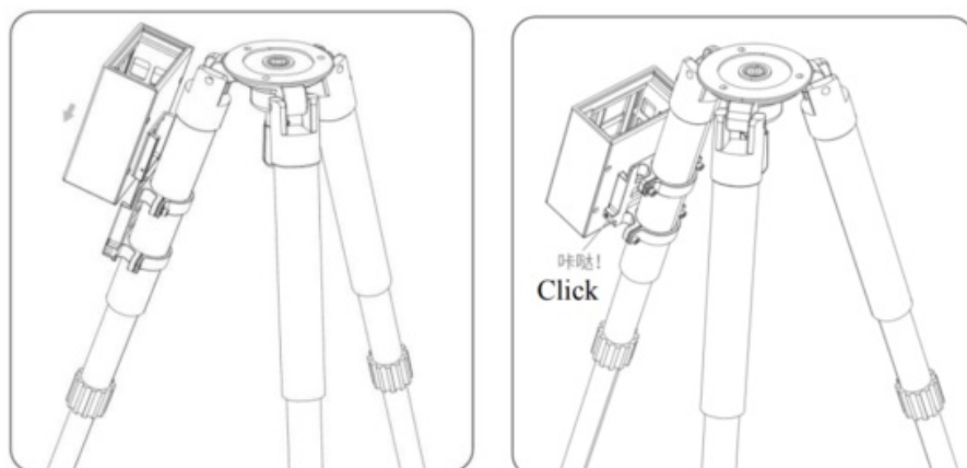
Figure 3-2.7 Installation diagram of HD TLS360 battery compartment
