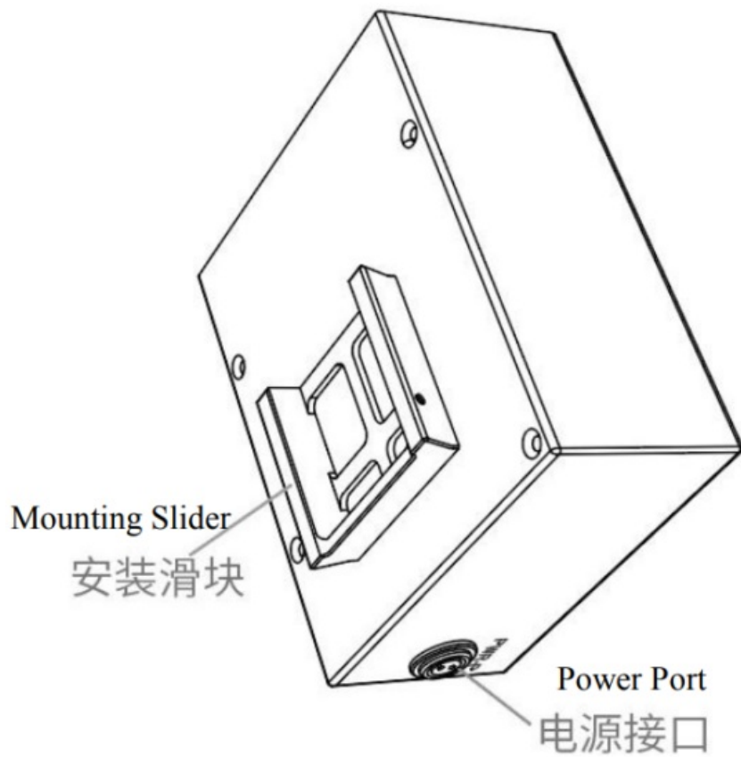
Figure 2-4 HD TLS360 system battery compartment
