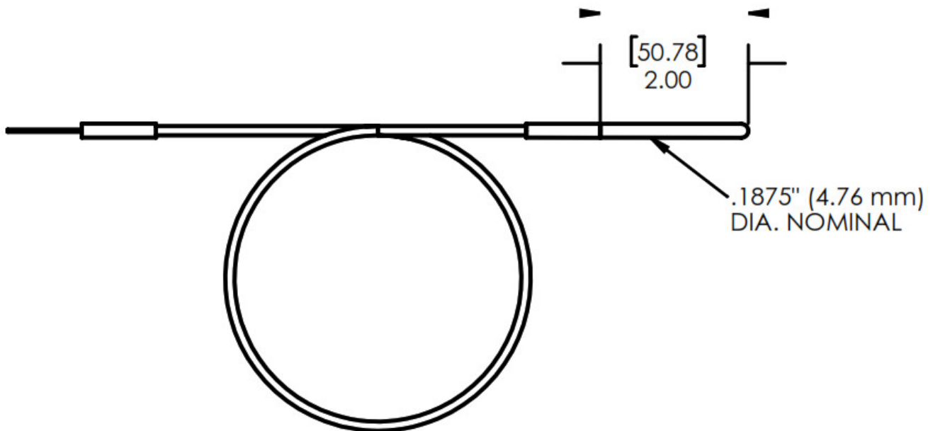
FIGURE 1: FREEZER PROBE DIMENSIONS
