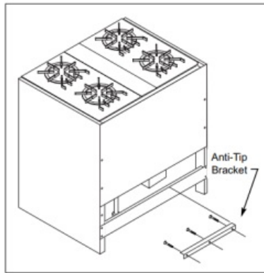
Figure 3-2. Anti-Tip Wall Bracket Installation
