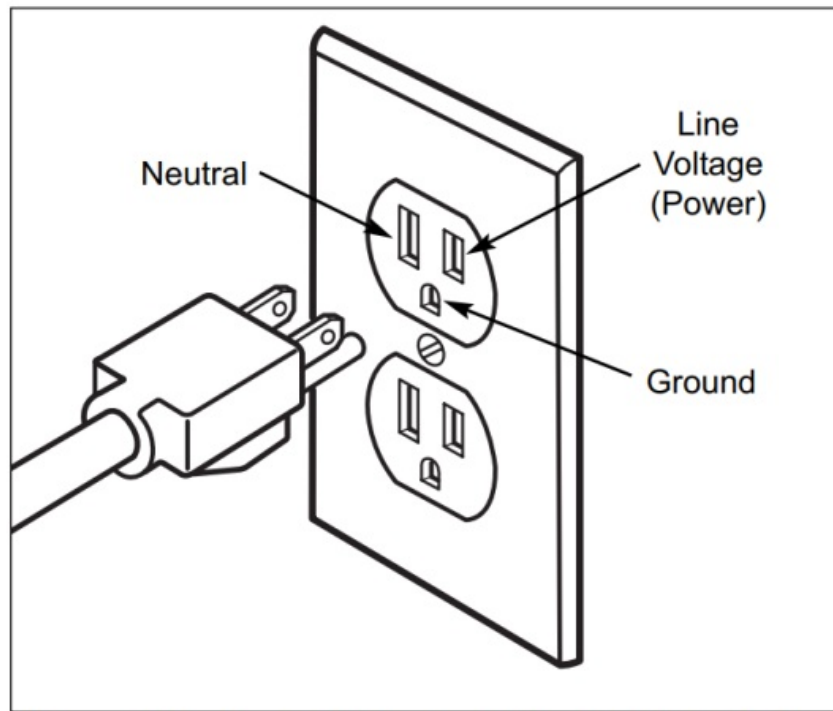
Figure 3-1. Proper Polarity at Electric Receptacle
