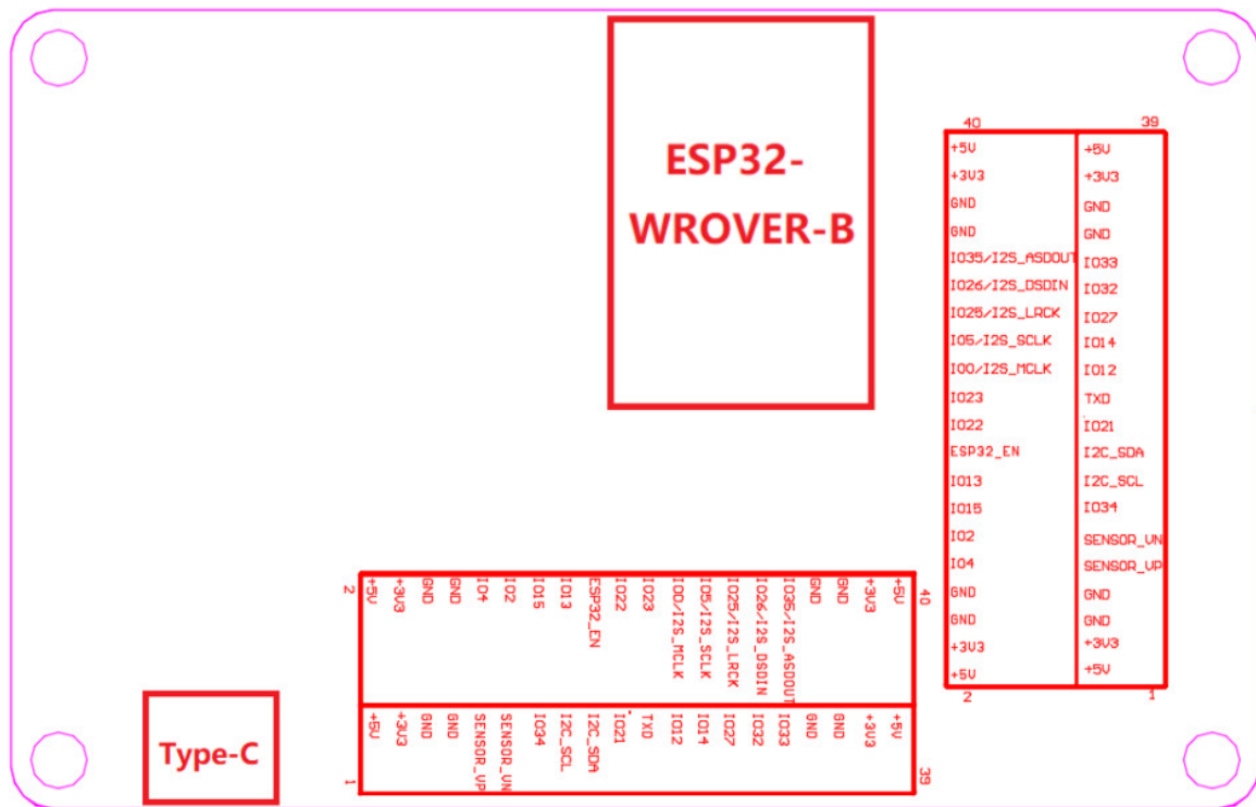
Figure 4: WT32-SC01 Interface Definition Diagram
