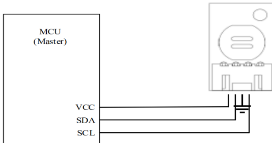
Figure 5 Typical application circuit
