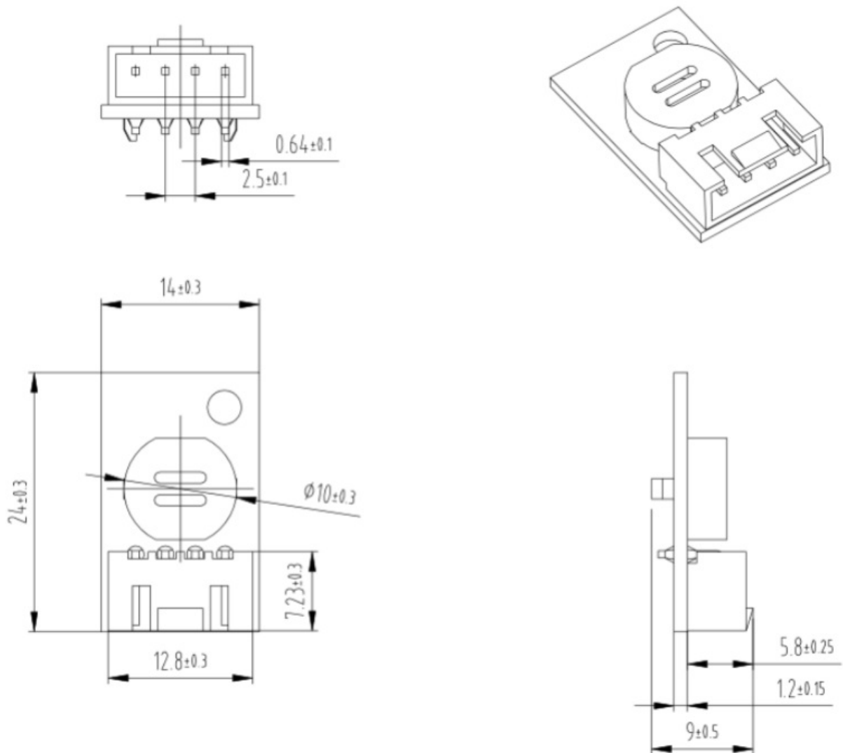
Figure 6 Product structure diagram (unit: mm)
