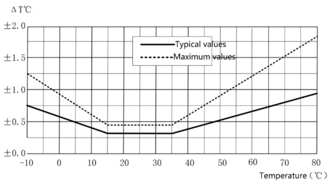
Fig 2 Temperature typical error and maximum error
