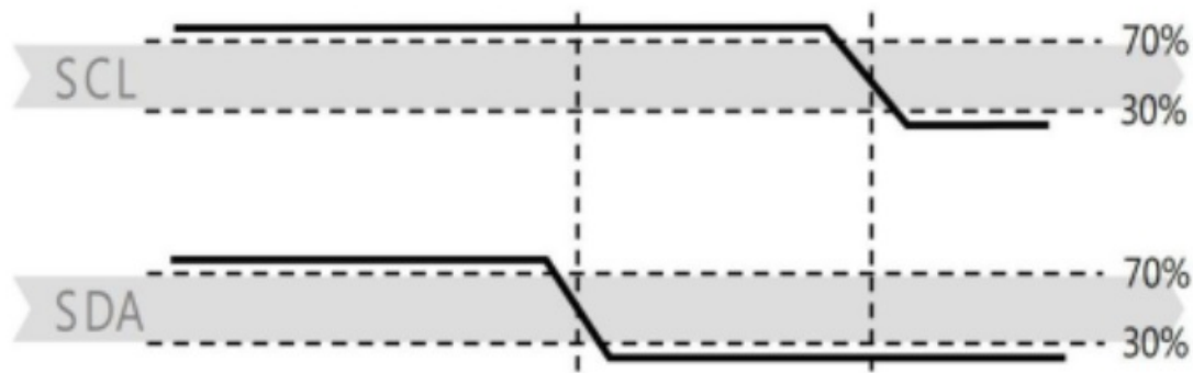
Figure 3 Start transmission state (S)
