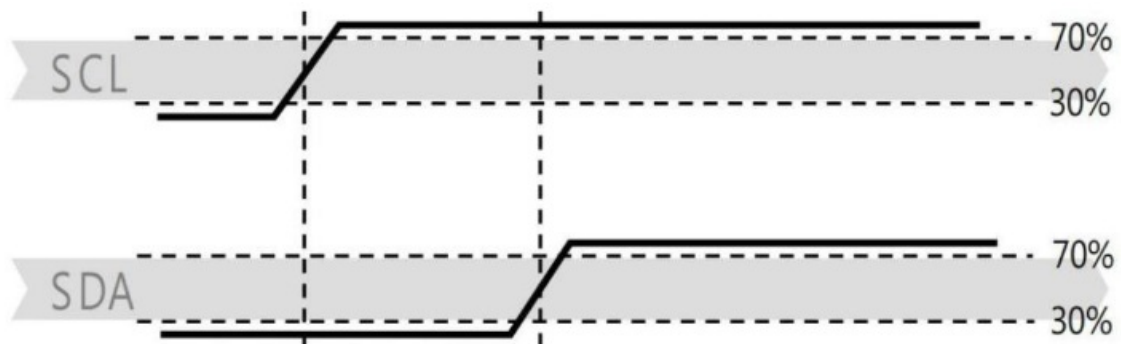
Figure4 Stop transmission state (P)
