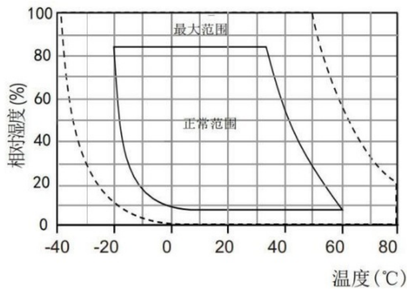
Figure 7 Working scope
