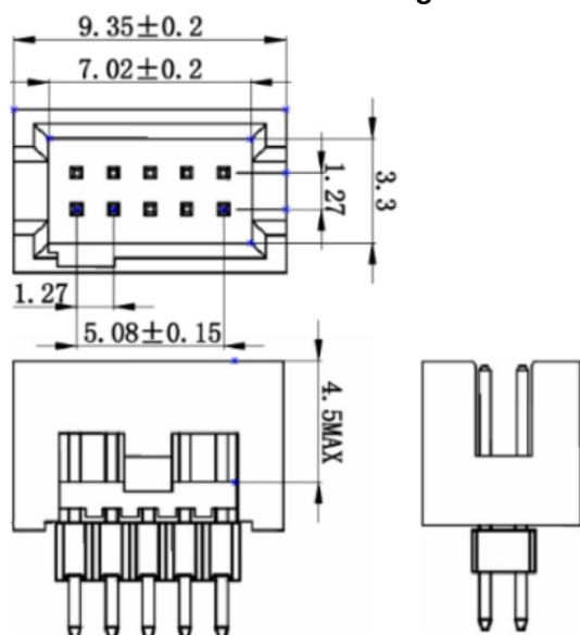
Figure 2-Terminal Model (PH=2x5x1.27mm)
