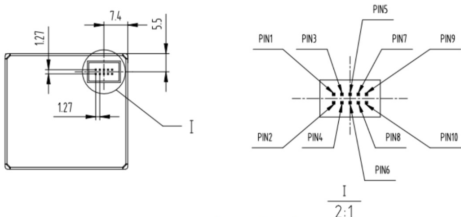
Figure1-Pin Order
