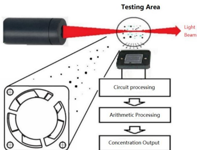
Figure 3-Principle Description
