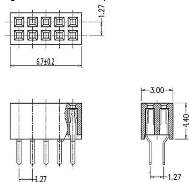
Figure 2-1 Mating terminals(for reference only)
