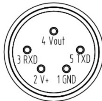
Picture 3. Pin Definition
