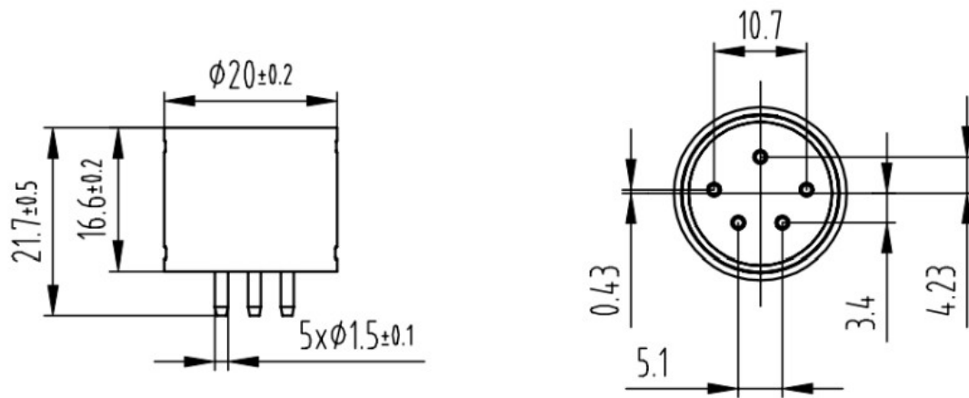
Picture 2: Sensor structure diagram
