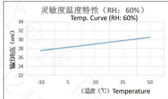
Fig6. Sensitivity at different temp.
