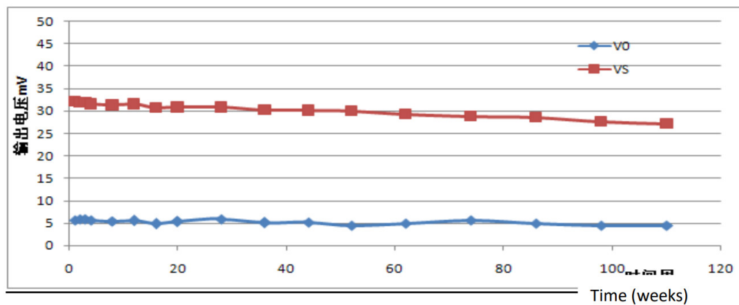
Fig11. Zero and Sensitivity stability curve
