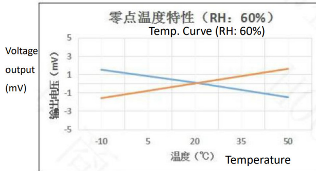
Fig5. Zero point at different temp.
