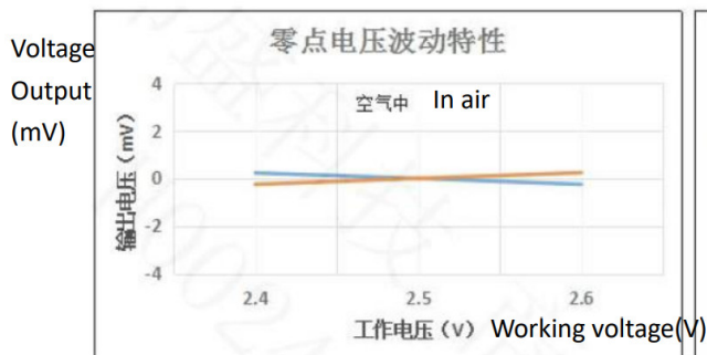
Fig9. Zero Drift with different voltage
