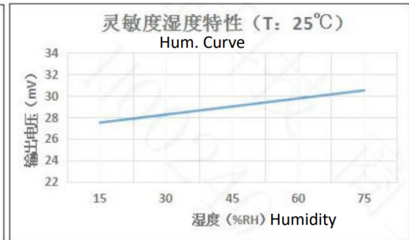
Fig8. Sensitivity at different humidity
