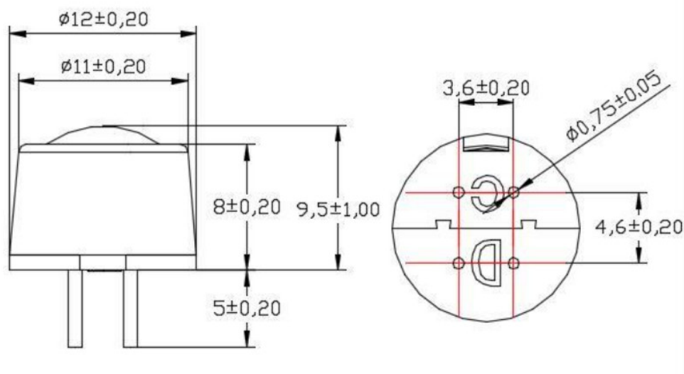
Fig1. Sensor Structure
