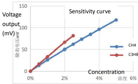
Fig3. Sensitivity Curve
