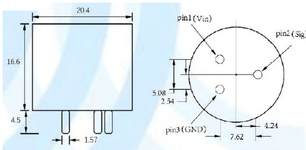
Fig2.Dimension (unit: mm)
