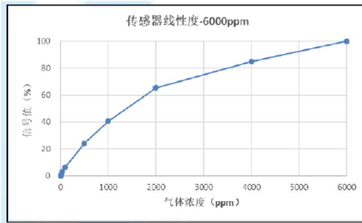
Fig4. Typical linear output curve(6000ppm)
