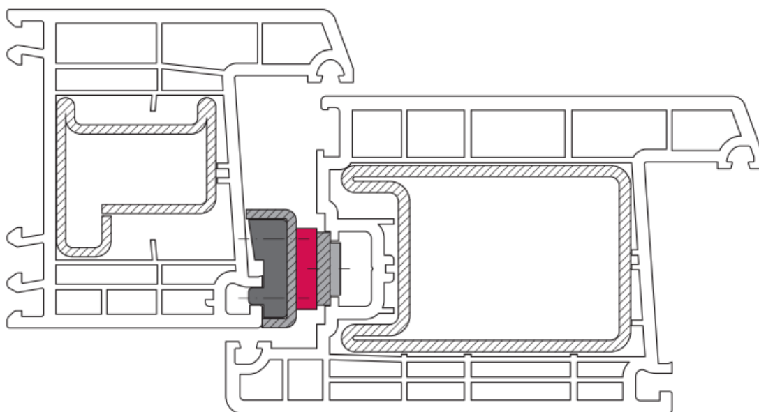
Section A-A (keep rail)
