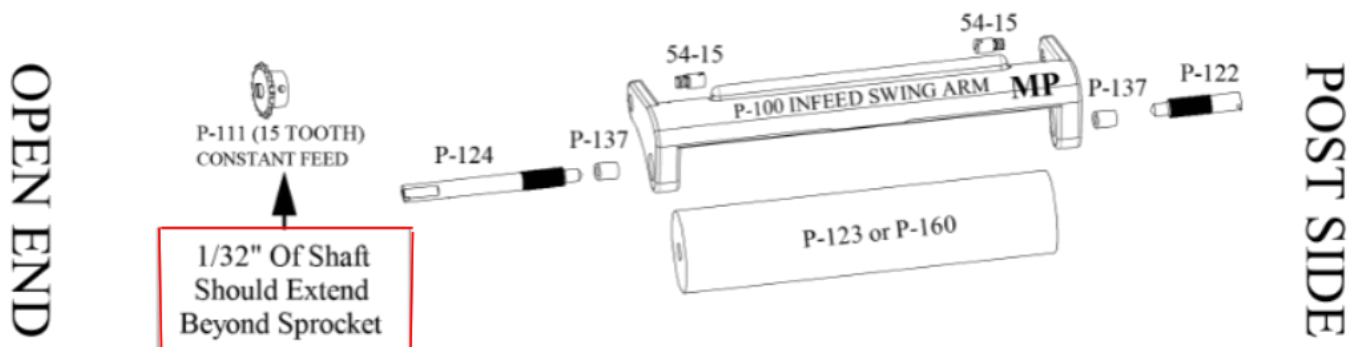
54-513 MULTI-PASS INFEEED SWING ARM ASSEMBLY
