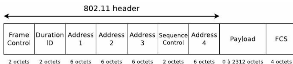
Fig. 1: Structure of a 802.11 frame.
