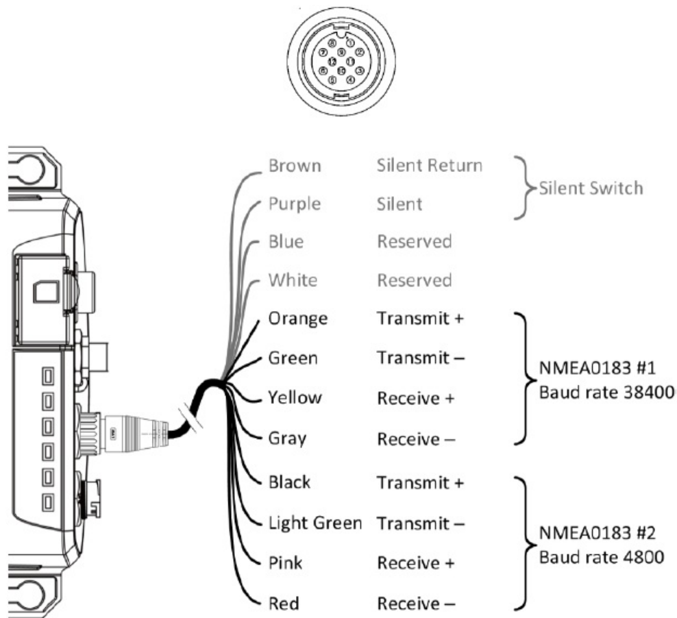
Figure 8 NMEA 0183 Connection
