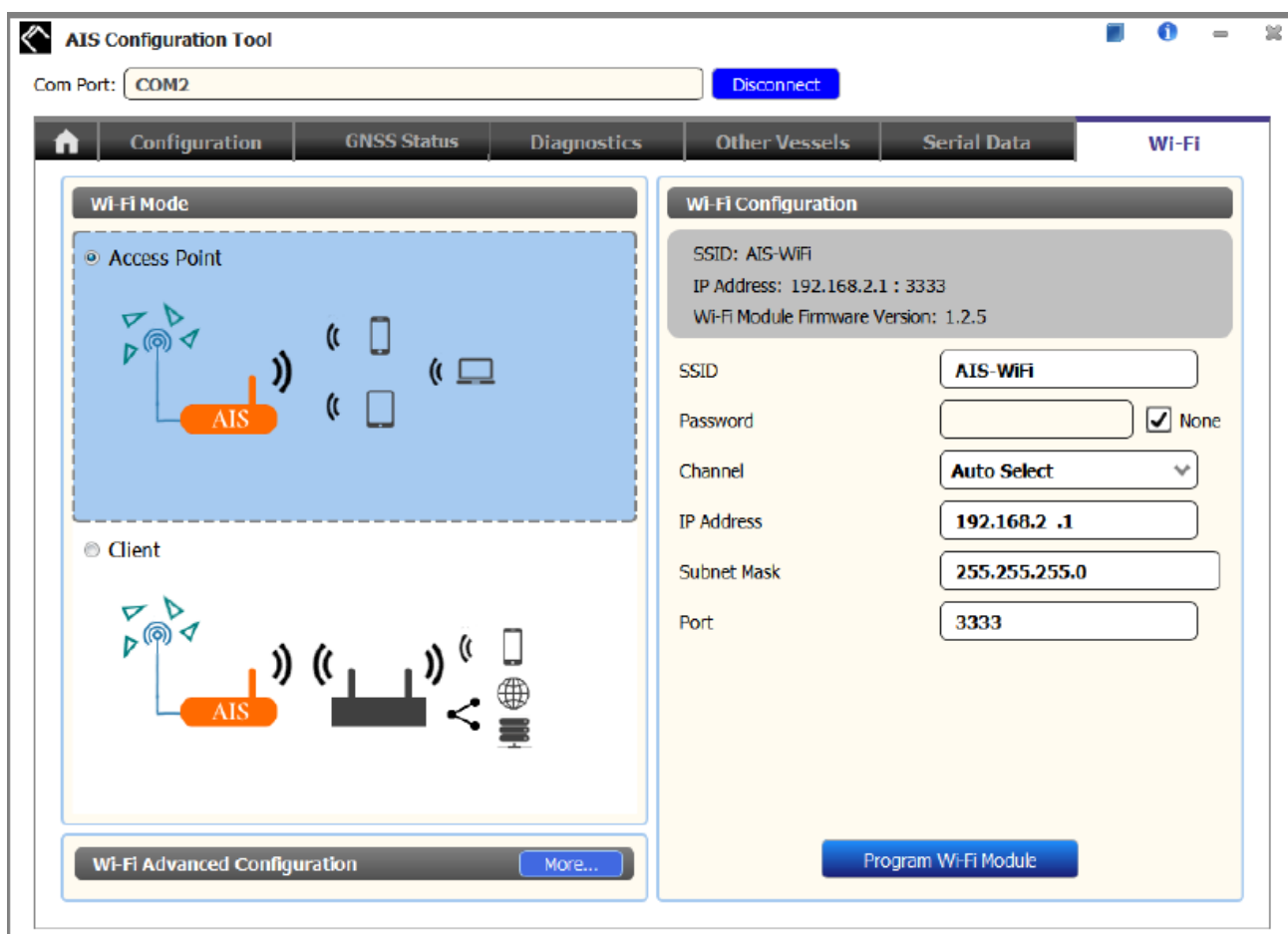
Figure 14 Access Point Mode
