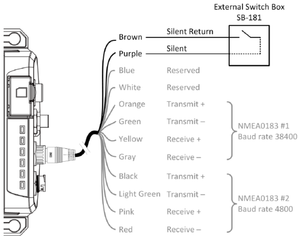
Figure 9 Silent Switch Connection
