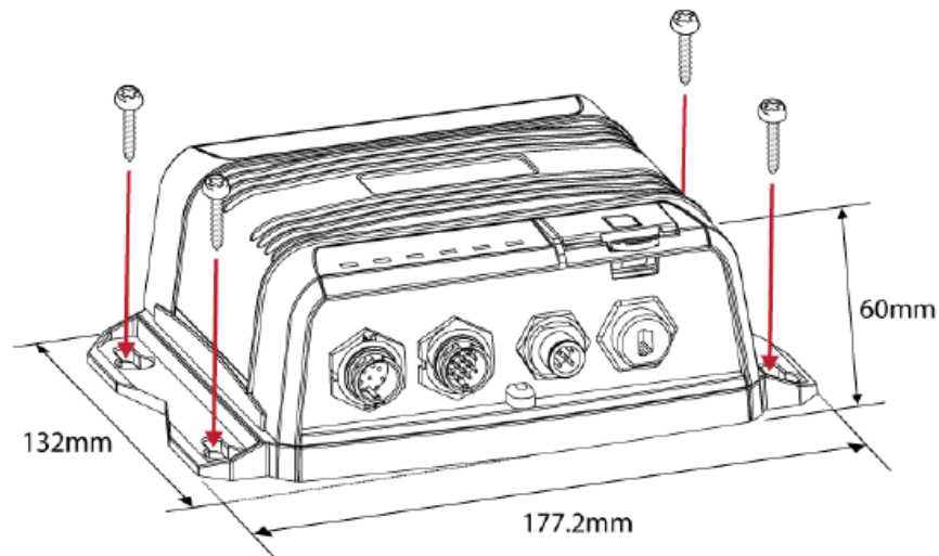
Figure 2 Mounting the Device
