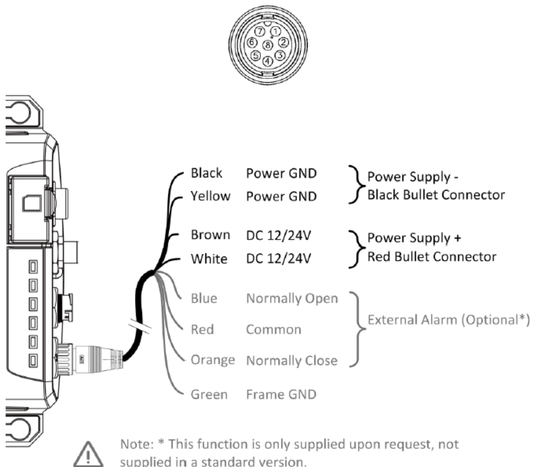
Figure 11 Power and Alarm Connection
