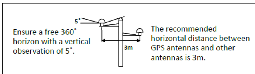
Figure 7 GPS Antenna Locations
