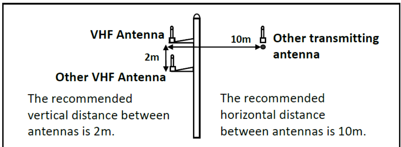
Figure 3 VHF Antenna Locations
