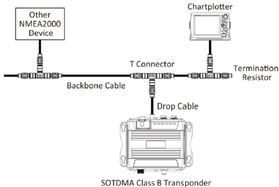
Figure 10 NMEA 2000 Network
