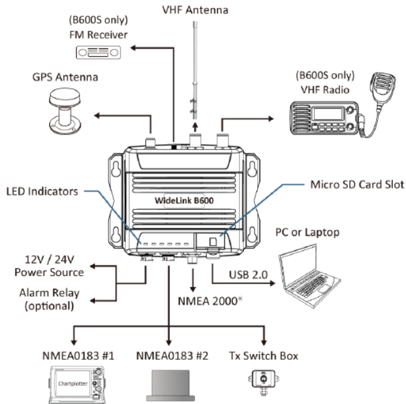
Figure 1 External Connections
