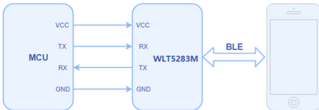
Figure 4-2: UART communication
