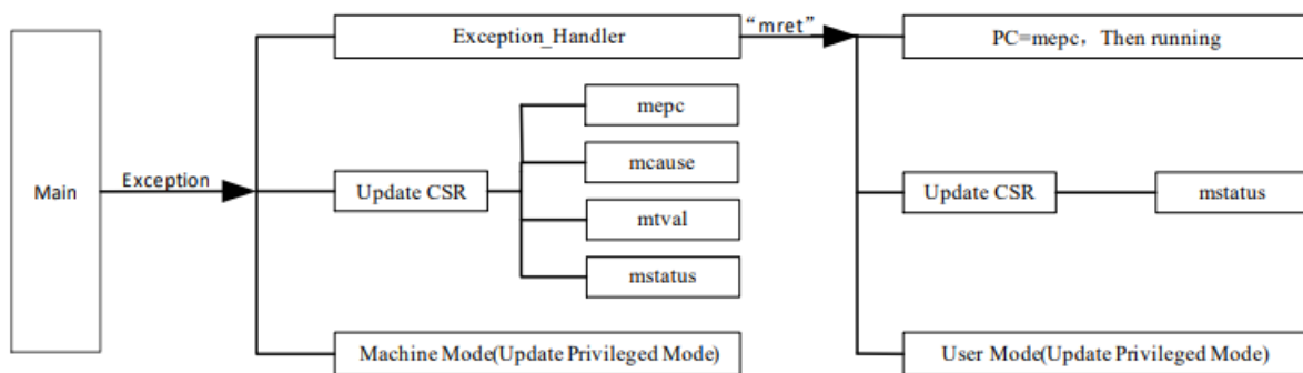
Figure 2-1 Exception response process diagram
