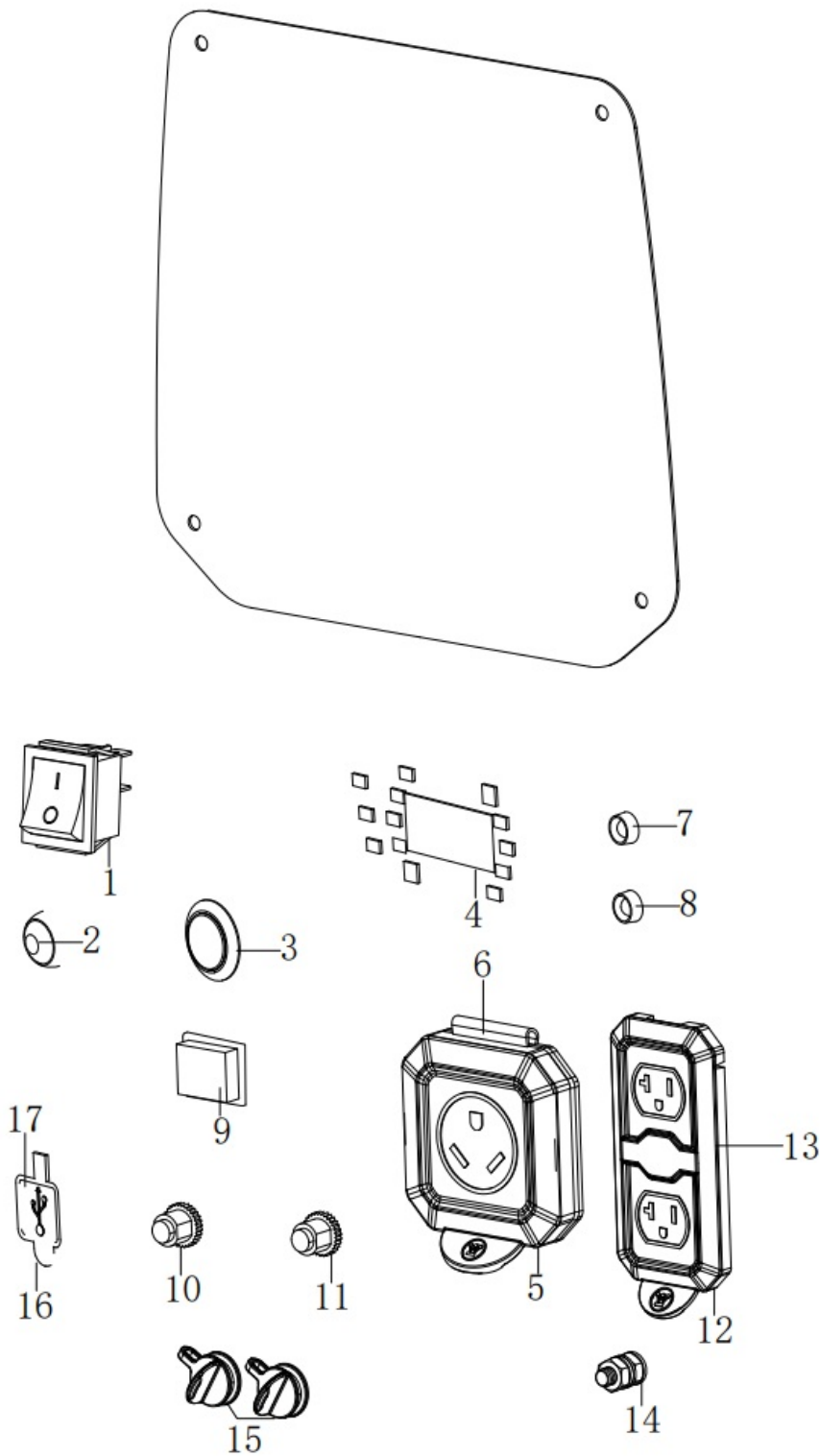
Parts List B (Control Panel)
