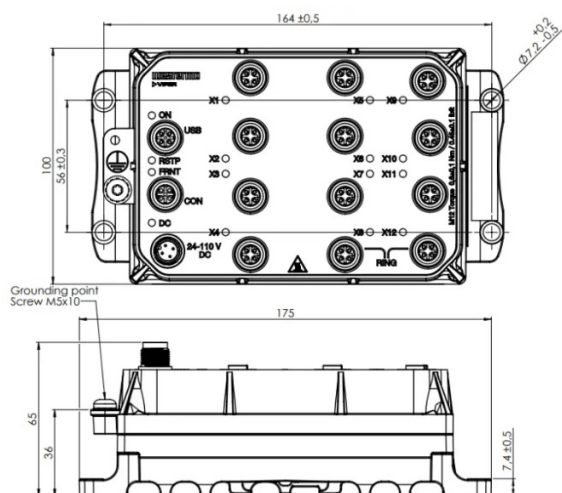
Figure 4. Dimensional drawing
