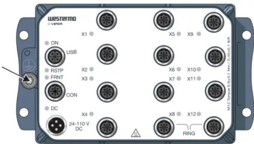
Figure 6. Earth connection
